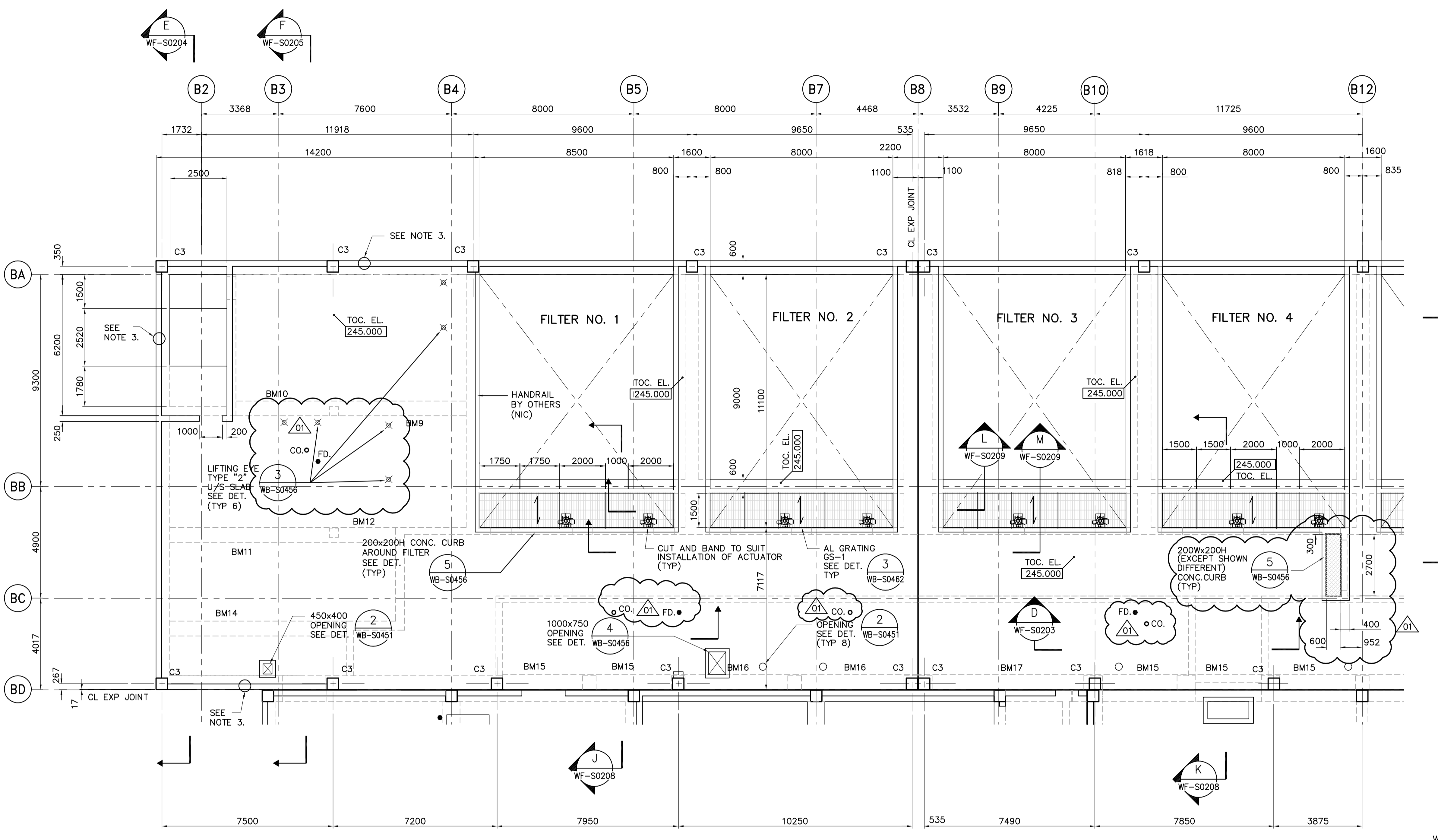
THIRD FLOOR PLAN AT EL. 245.000 1:100
