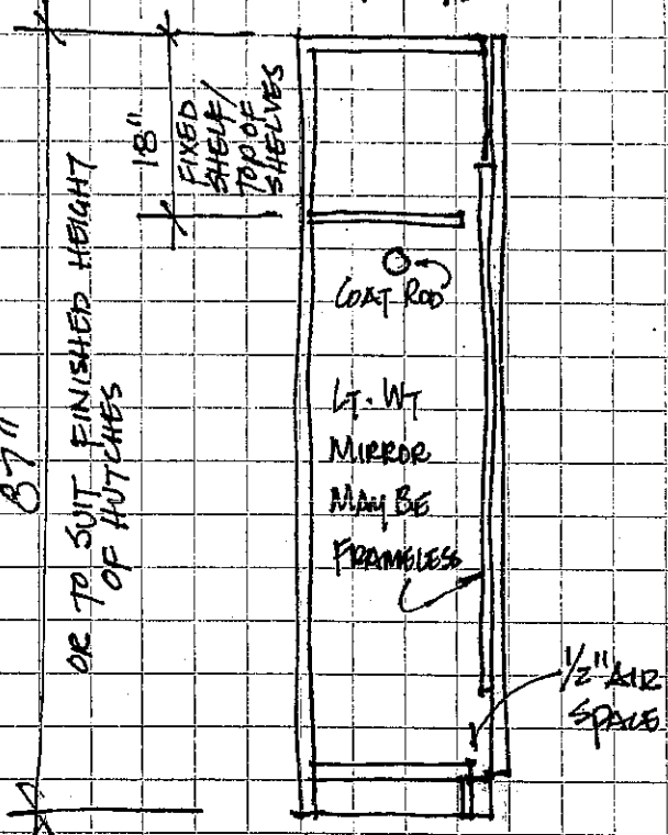
"A" SECTION THRU COATS
