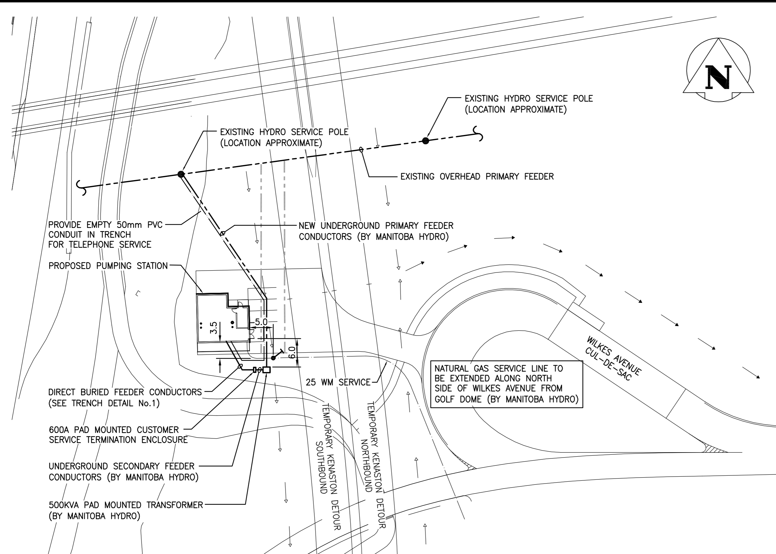
ELECTRICAL SITE PLAN 1:500
