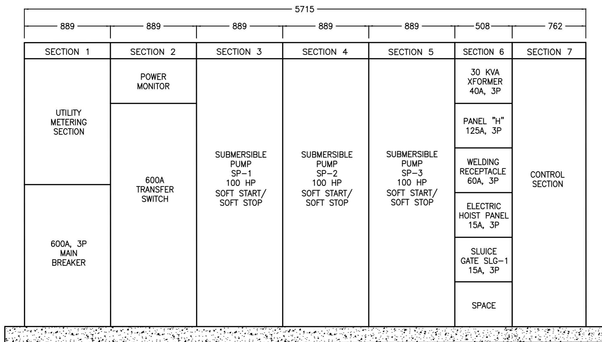
MCC PROPOSED LAYOUT N.T.S.
