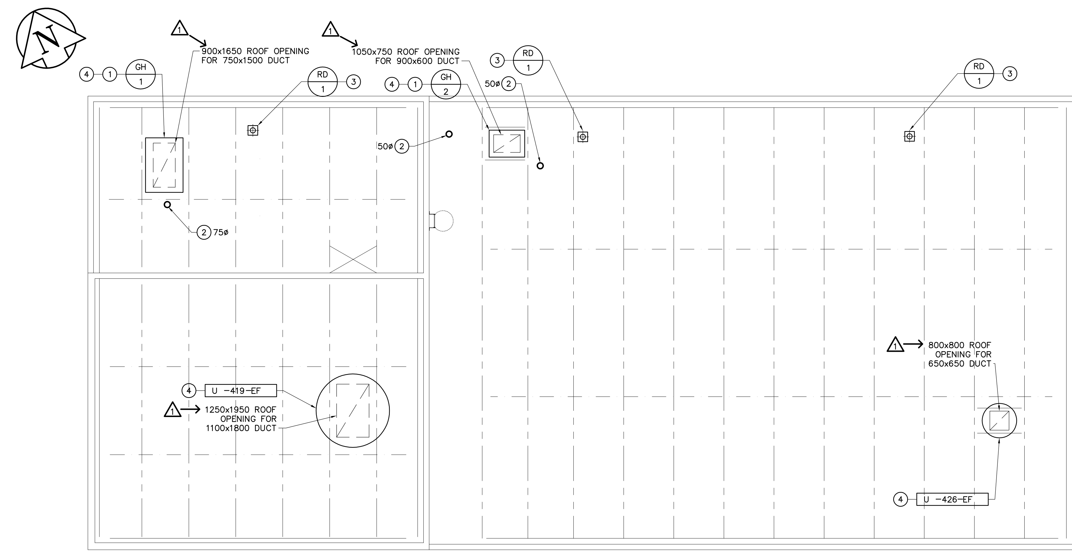
① PLAN VIEW – ROOF M4.02 SCALE 1:75
