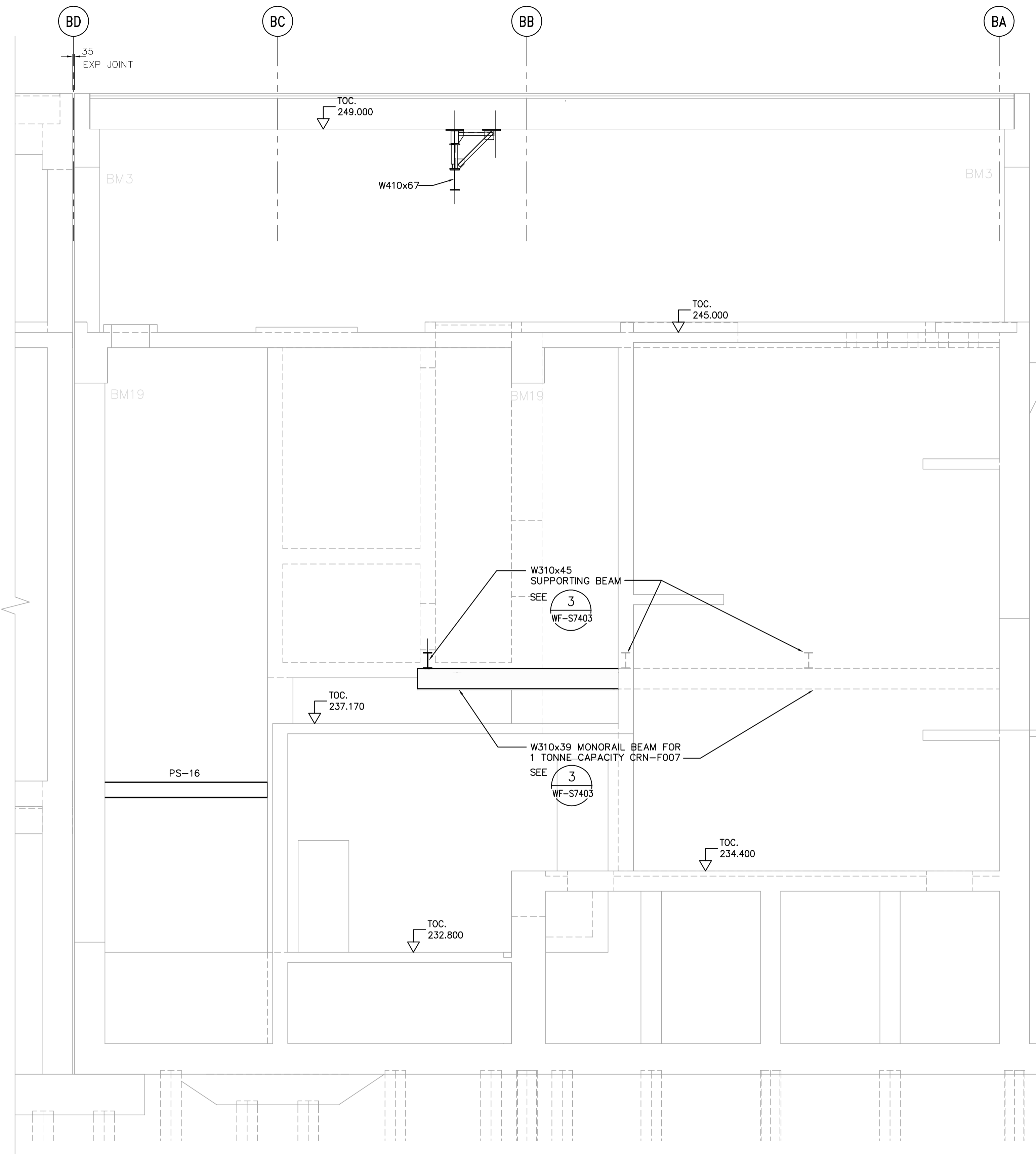
H SECTION WF-S7118 1:50 WF-S7147
