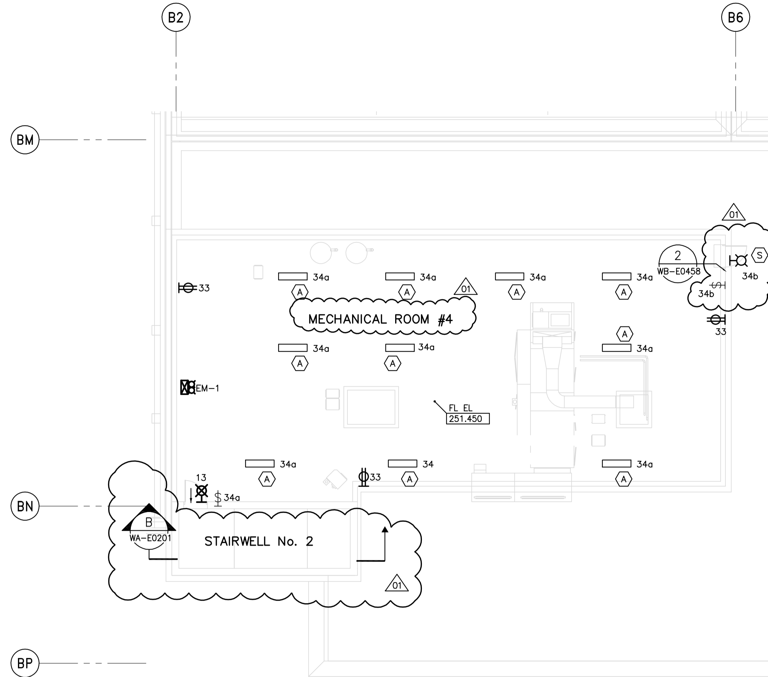
MECHANICAL ROOM #4 POWER AND LIGHTING PLAN 1:100
