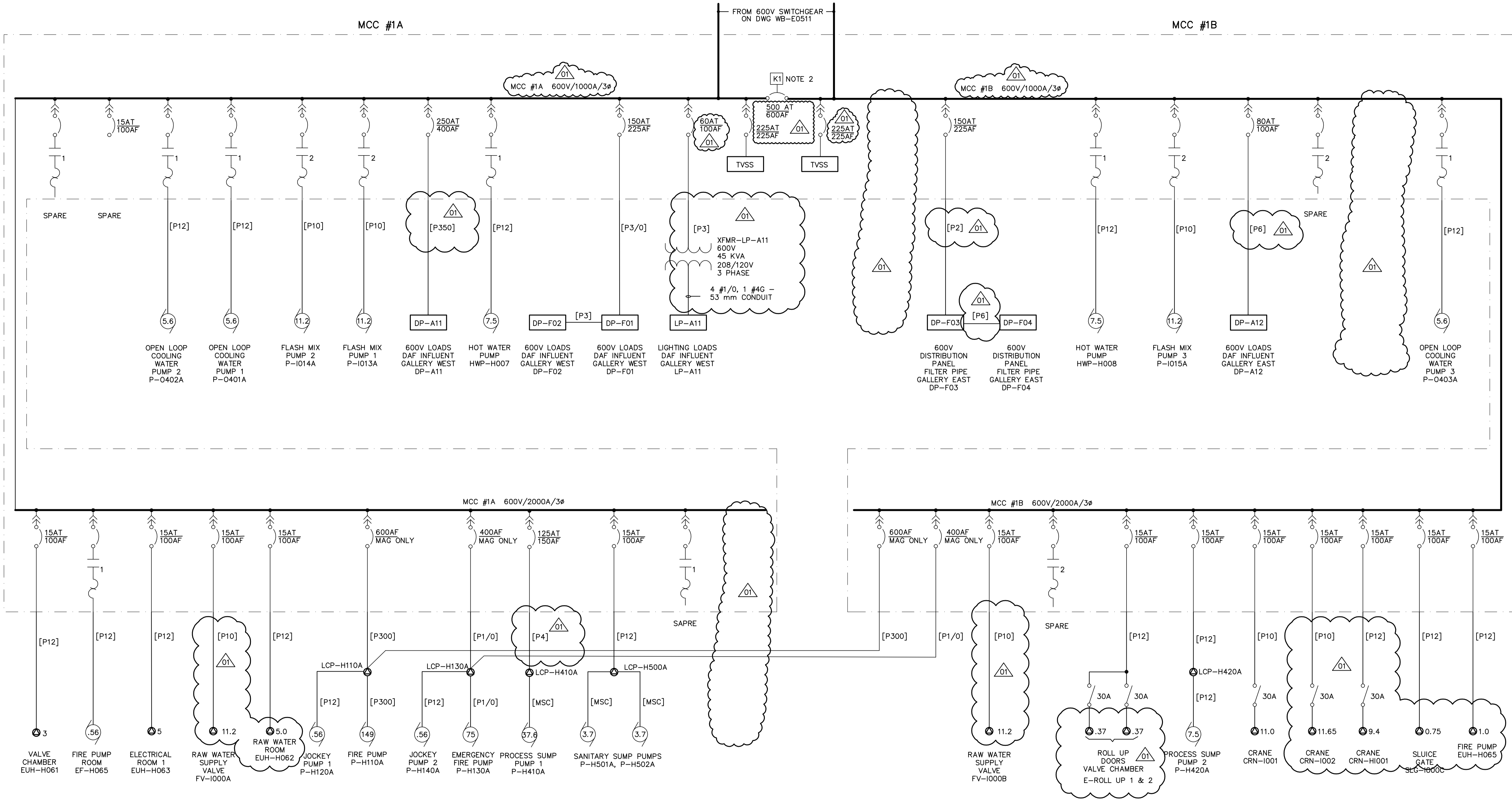
MCC #1A, #1B SINGLE LINE DIAGRAM
