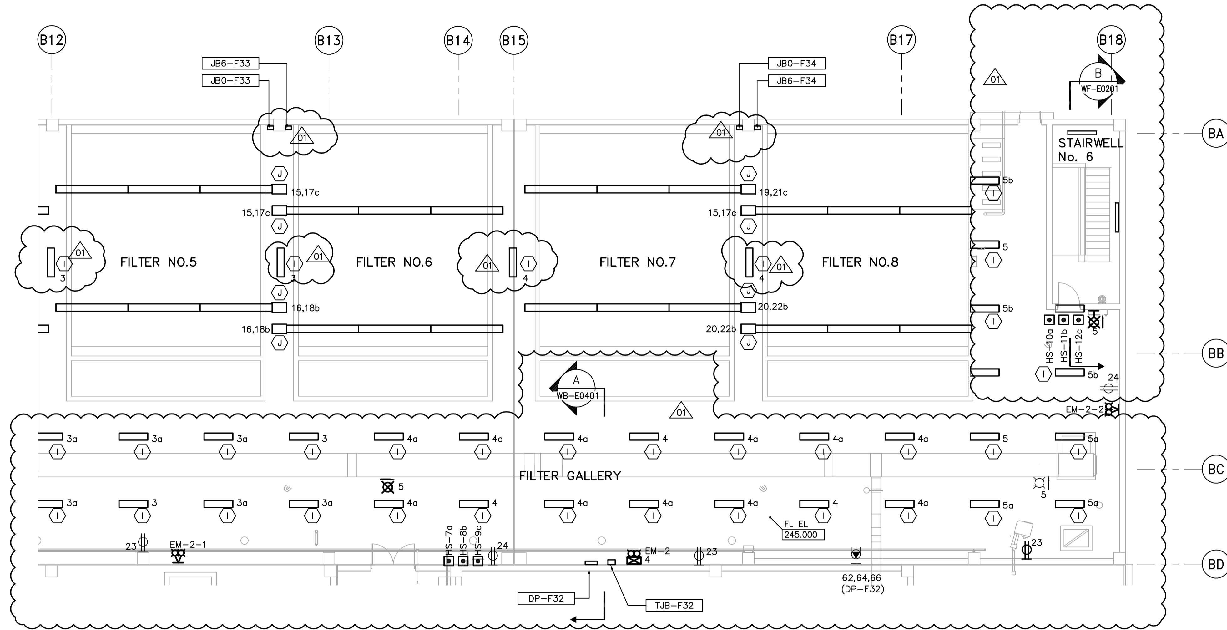
THIRD FLOOR POWER AND LIGHTING PLAN (AREA 2) 1:100
