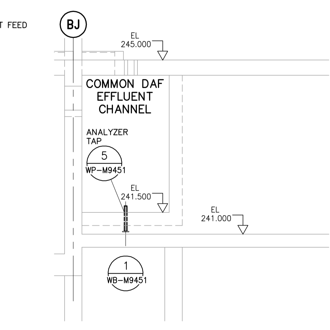
Q SECTION - EMBEDDED ANALYSER TAP TYP. 2 WP-M9101 1:50
