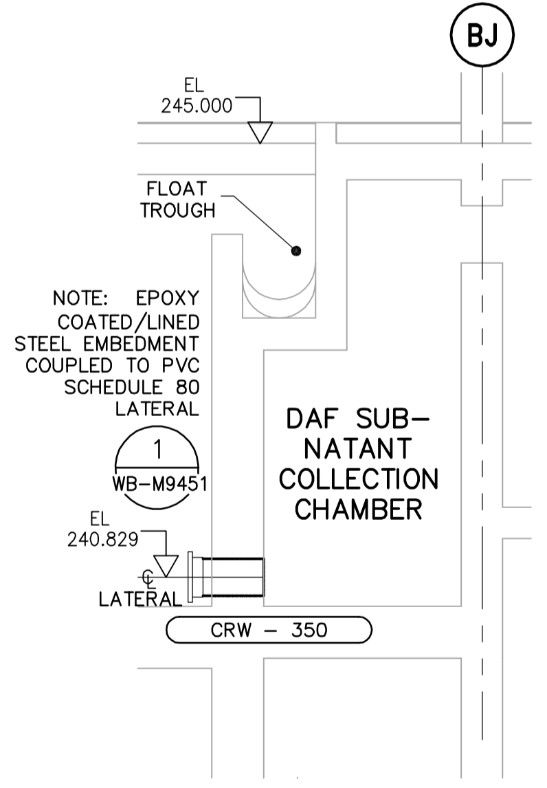
B SECTION - DAF LATERALS - TYP. 64 WP-M9101 1:50
