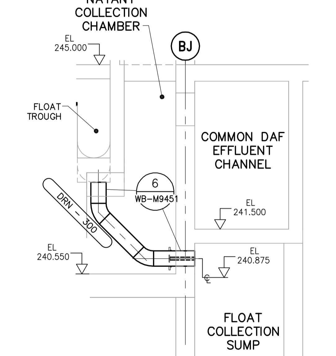
C SECTION - FLOAT TROUGH DRAINS TO FLOAT SUMPS TYP. 8 WP-M9101 1:50
