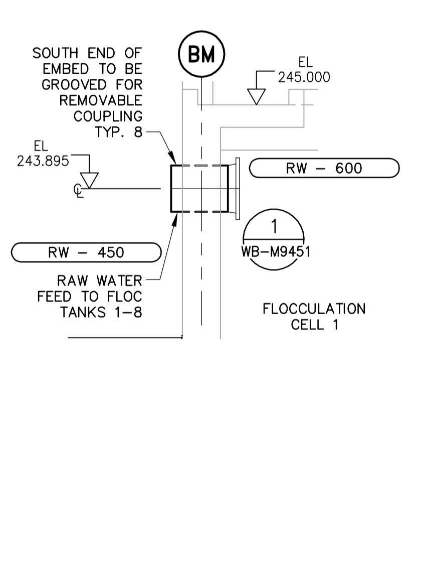
A SECTION - RAW WATER FEEDS TO FLOC TANKS - TYP. 8 WP-M9101 1:50
