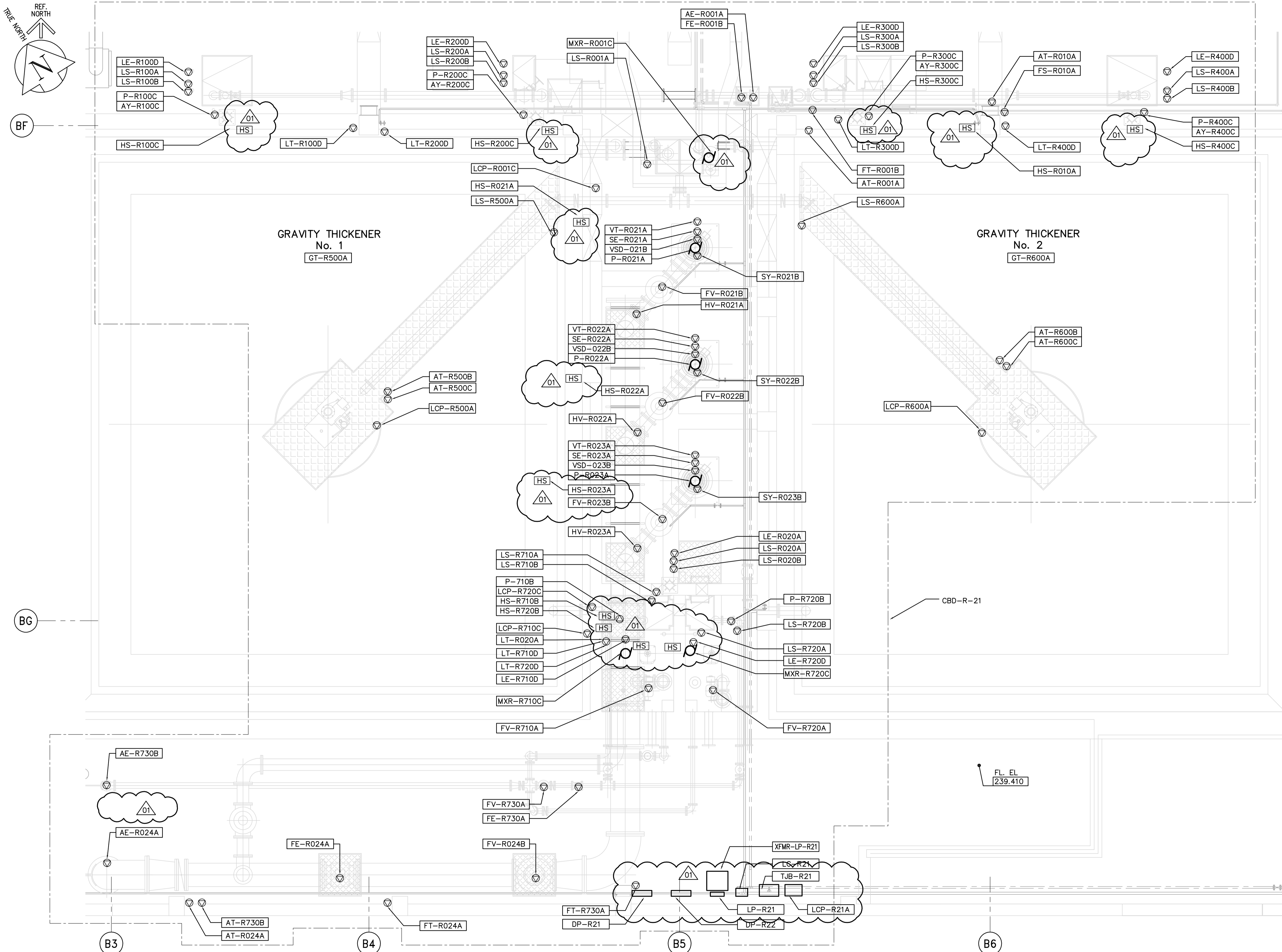
SECOND FLOOR PROCESS PLAN 1:100
