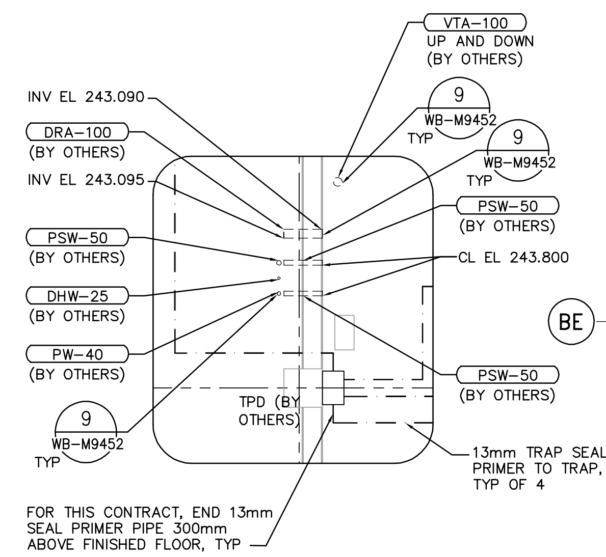
1 - 1:50 DETAIL
