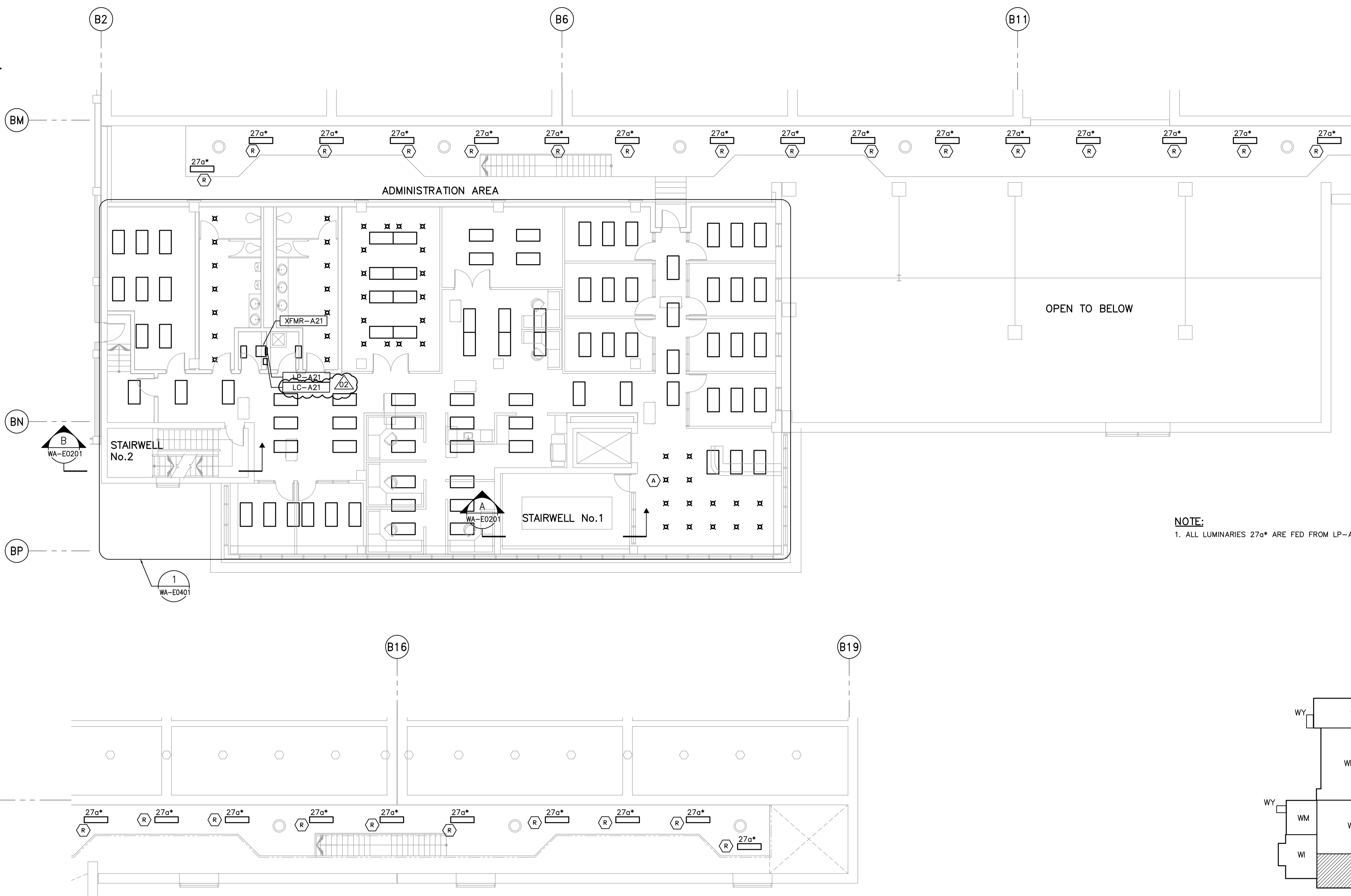
SECOND FLOOR POWER AND LIGHTING PLAN 1:100
