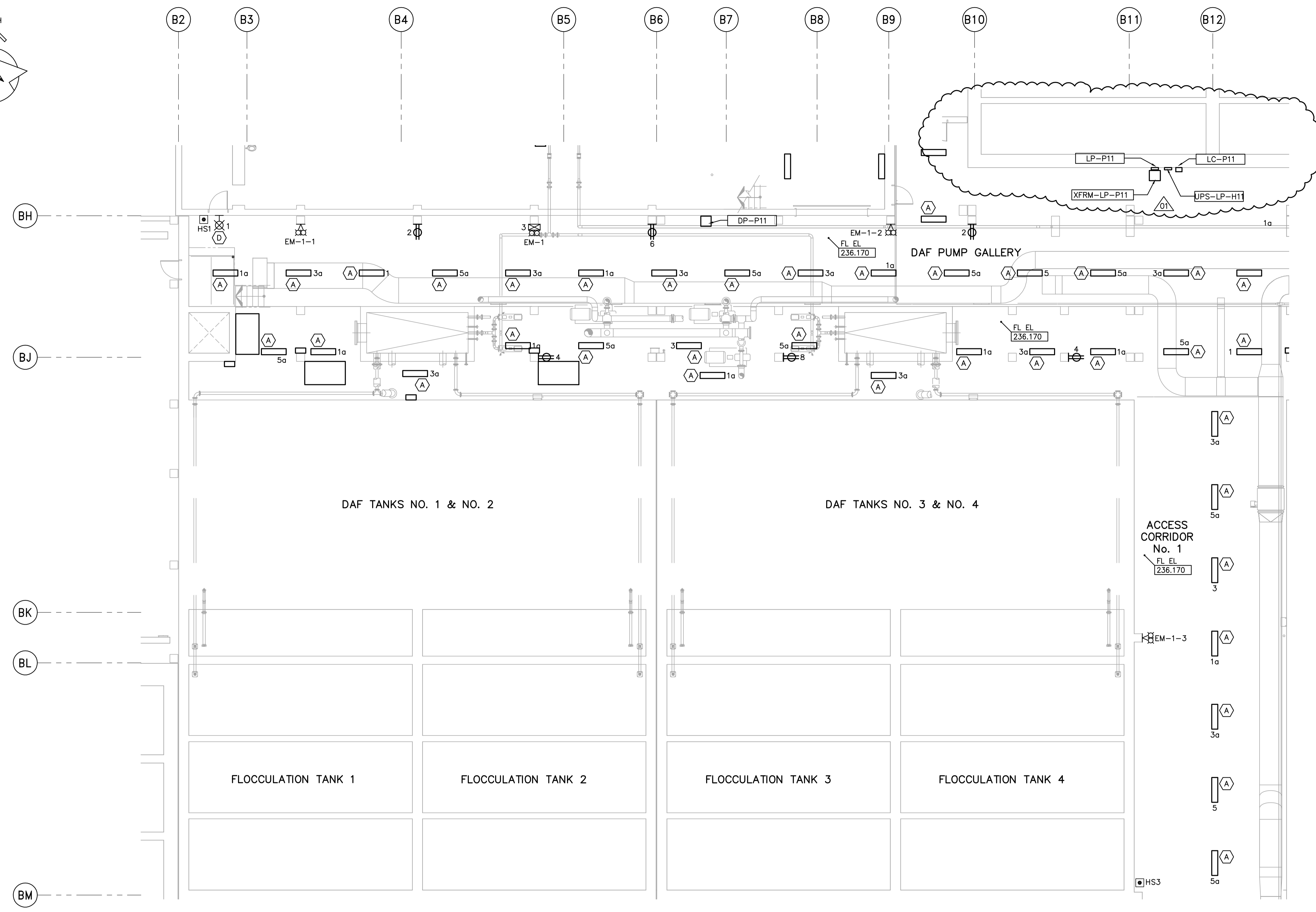
FIRST FLOOR POWER AND LIGHTING PLAN (AREA 1) 1:100
