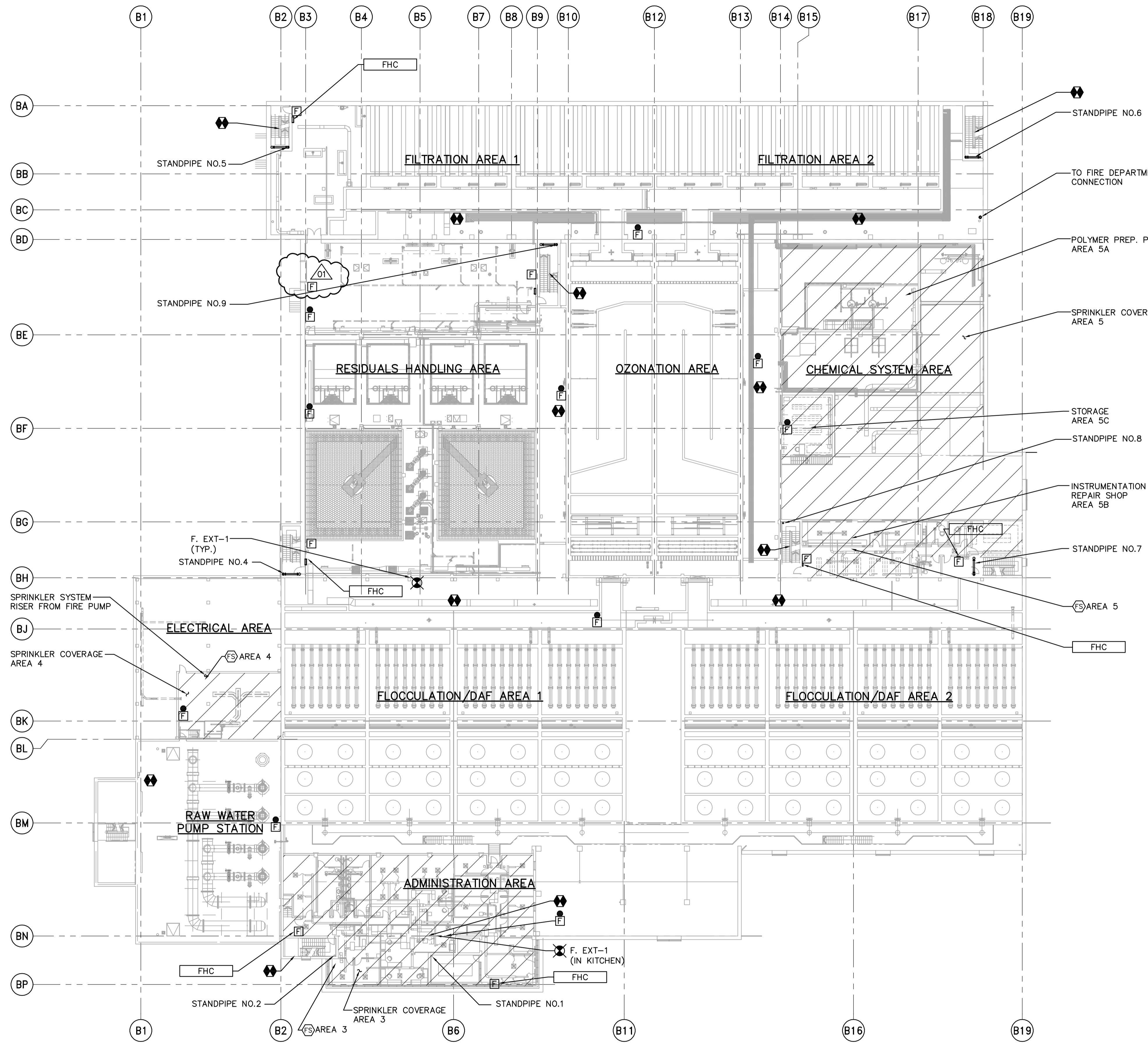
SECOND FLOOR PLAN 1:300
