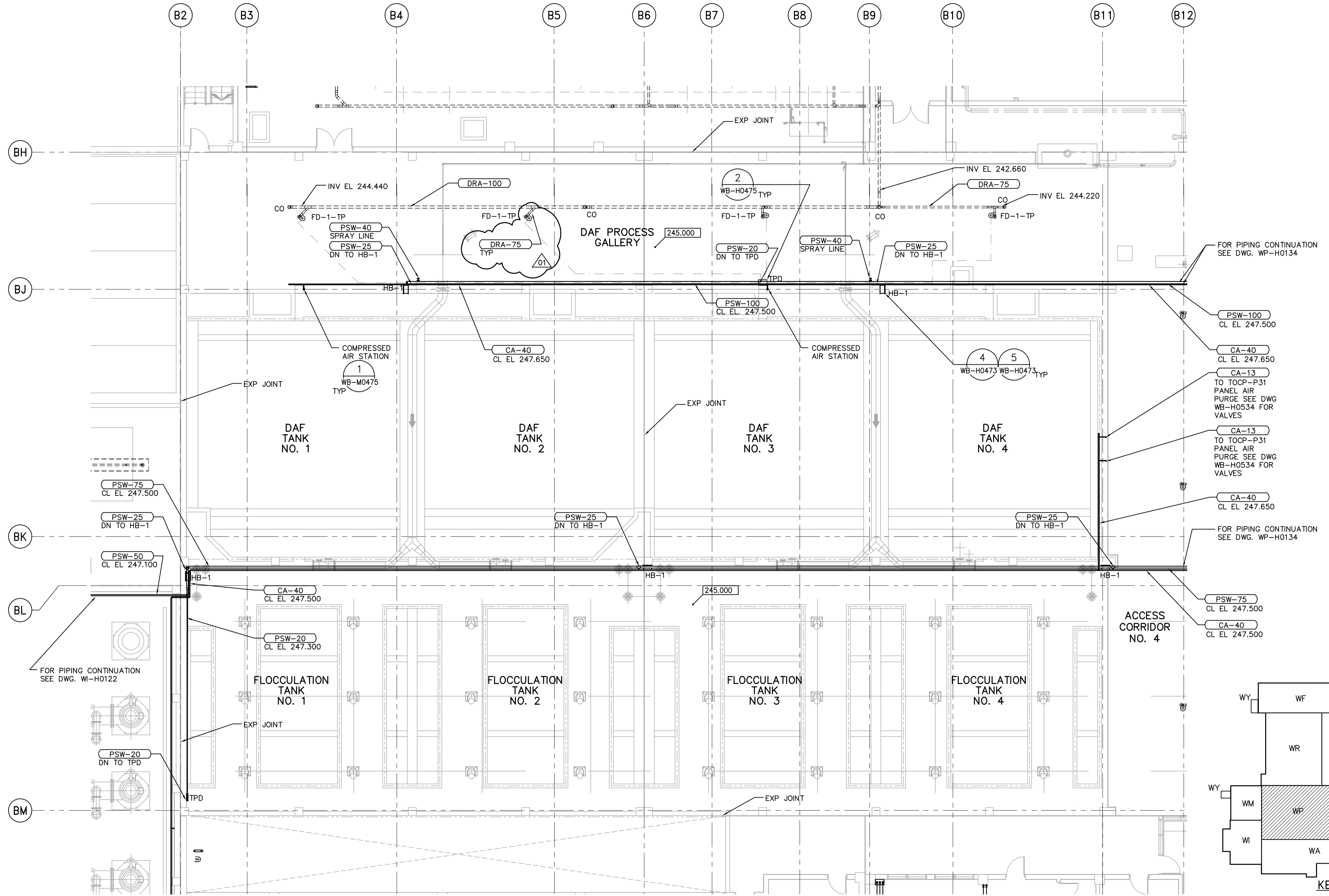
THIRD FLOOR PLAN 1:100
