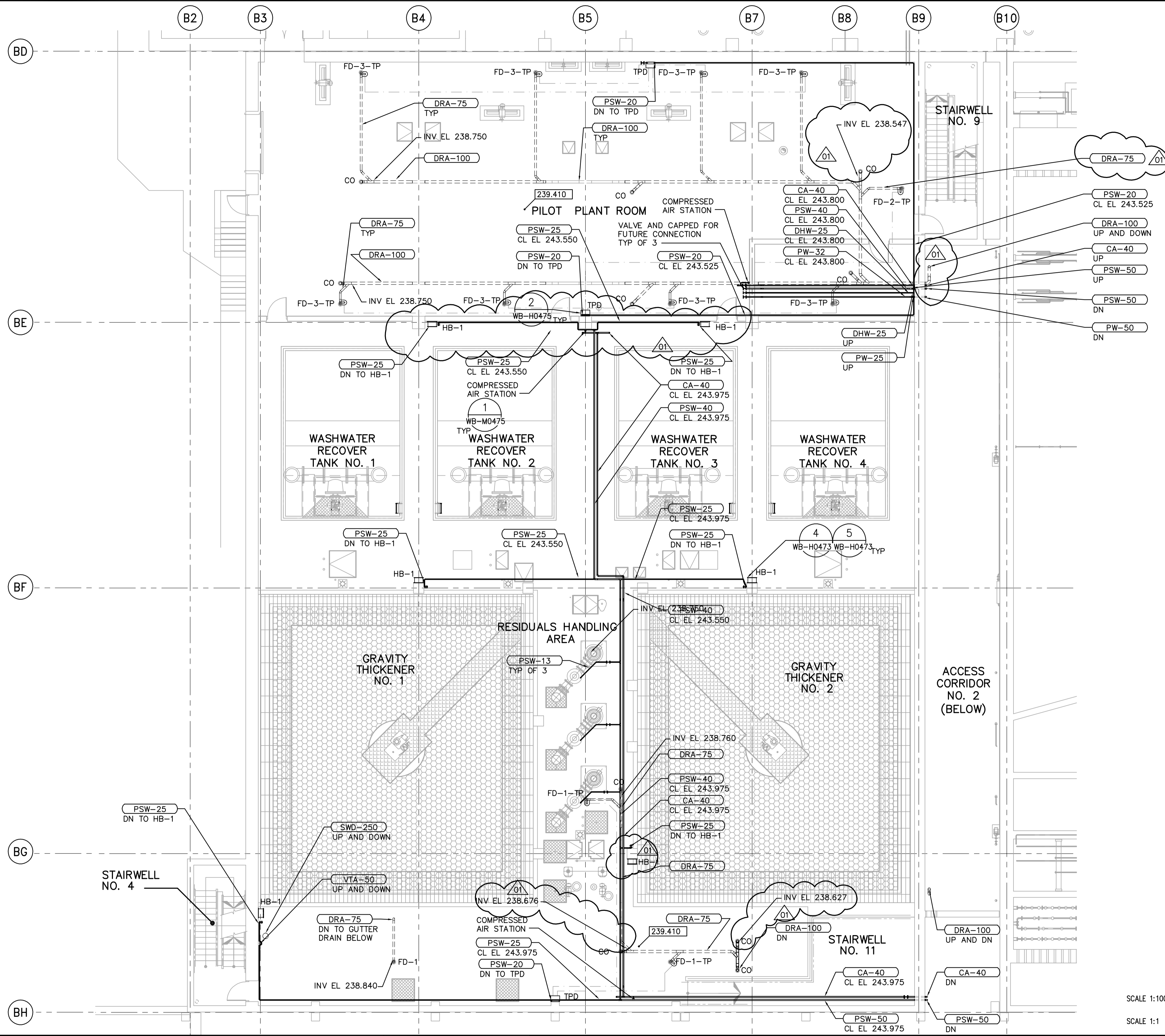
SECOND FLOOR PLAN 1:100
