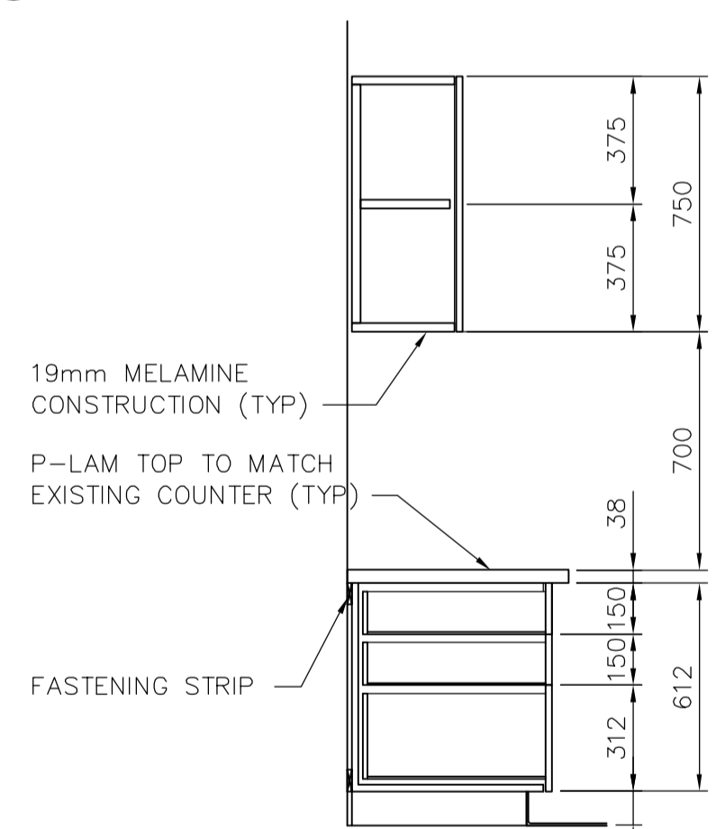
9 MILLWORK SECTION A1.01 1:20
