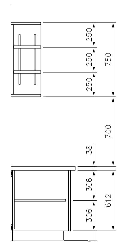
8 MILLWORK SECTION A1.01 1:20
