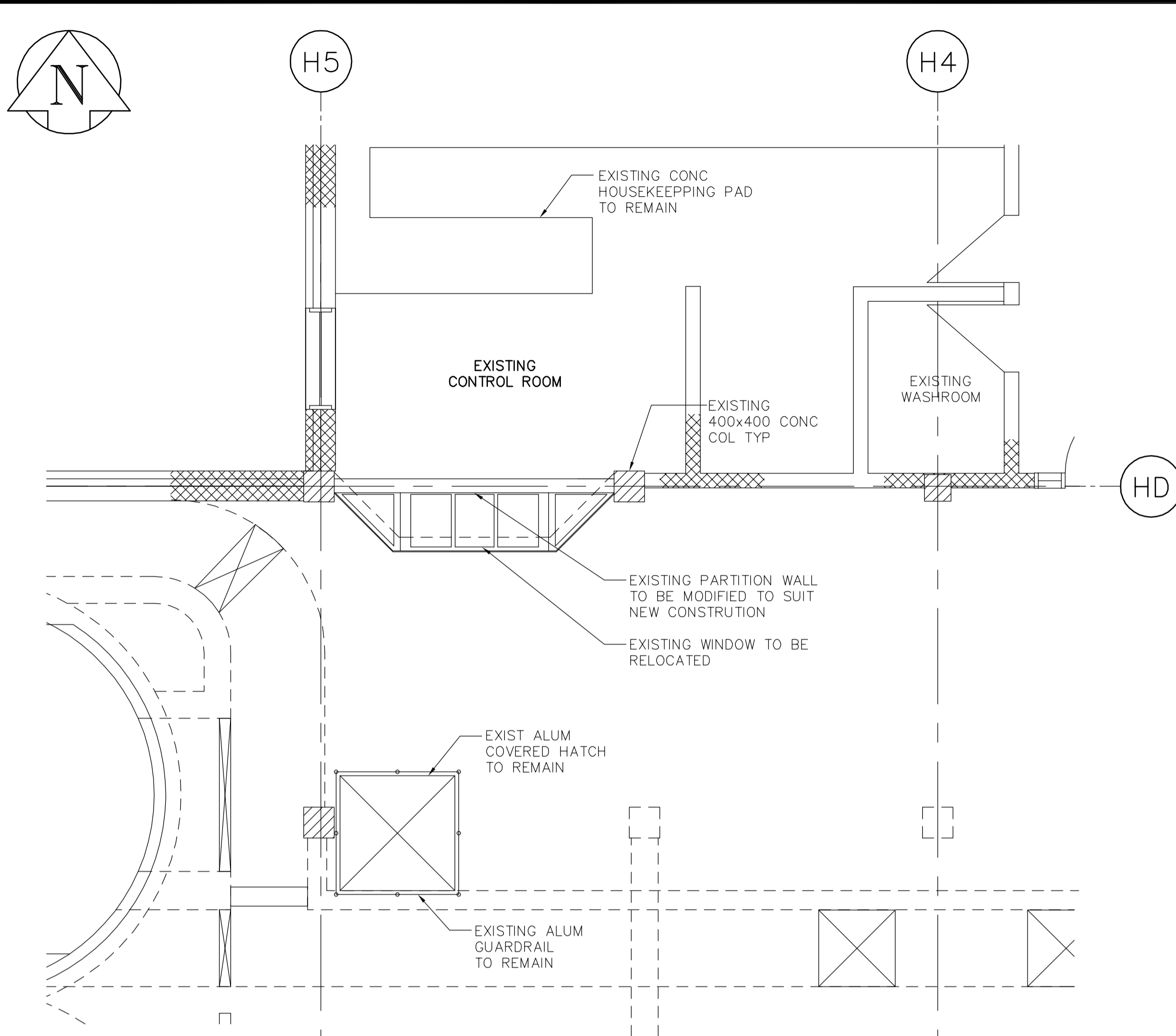
1 MAIN FLOOR DEMOLITION-PARTIAL PLAN A1.01 1:50
