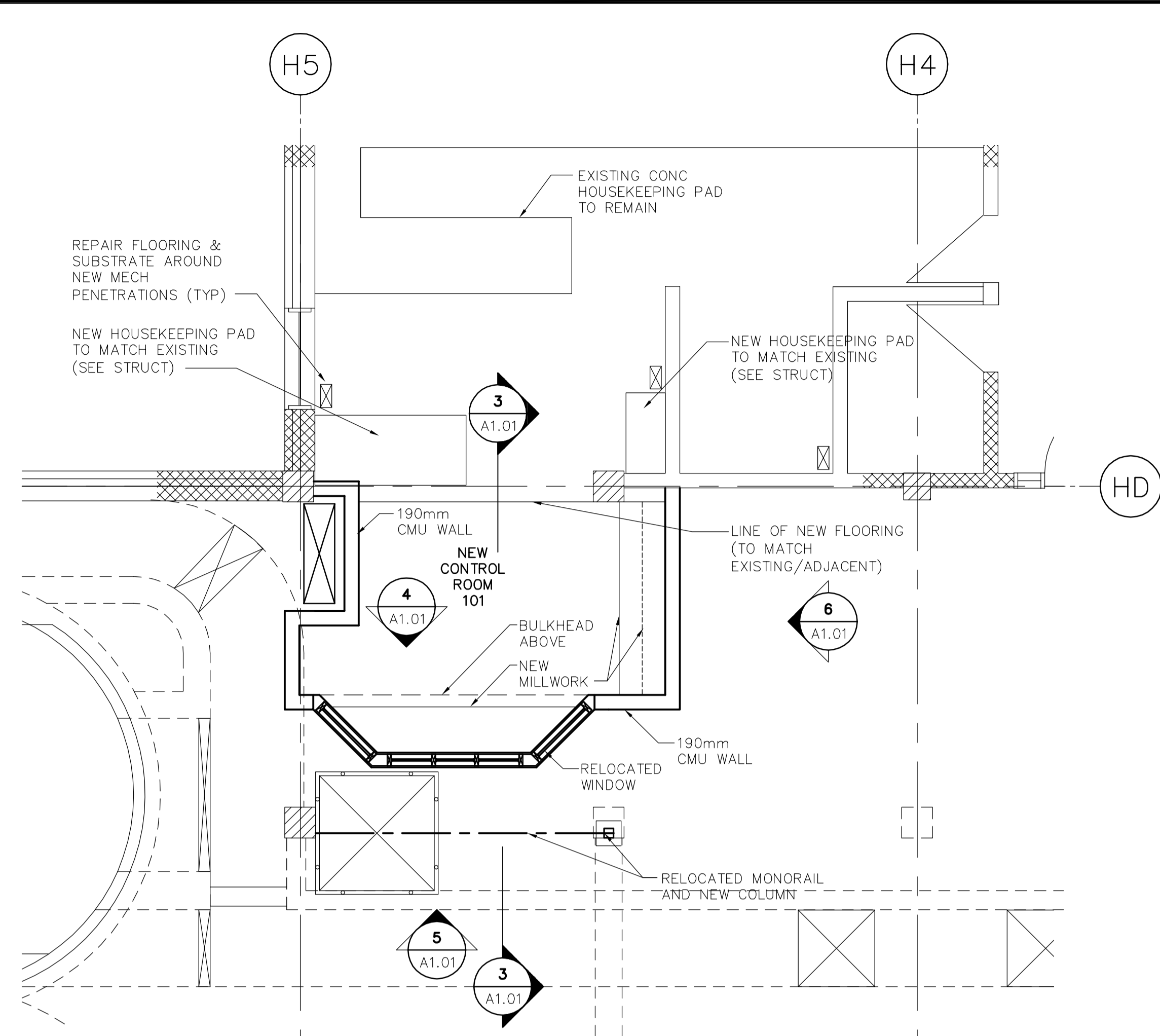
2 NEW MAIN FLOOR CONSTRUCTION-PARTIAL PLAN A1.01 1:50
