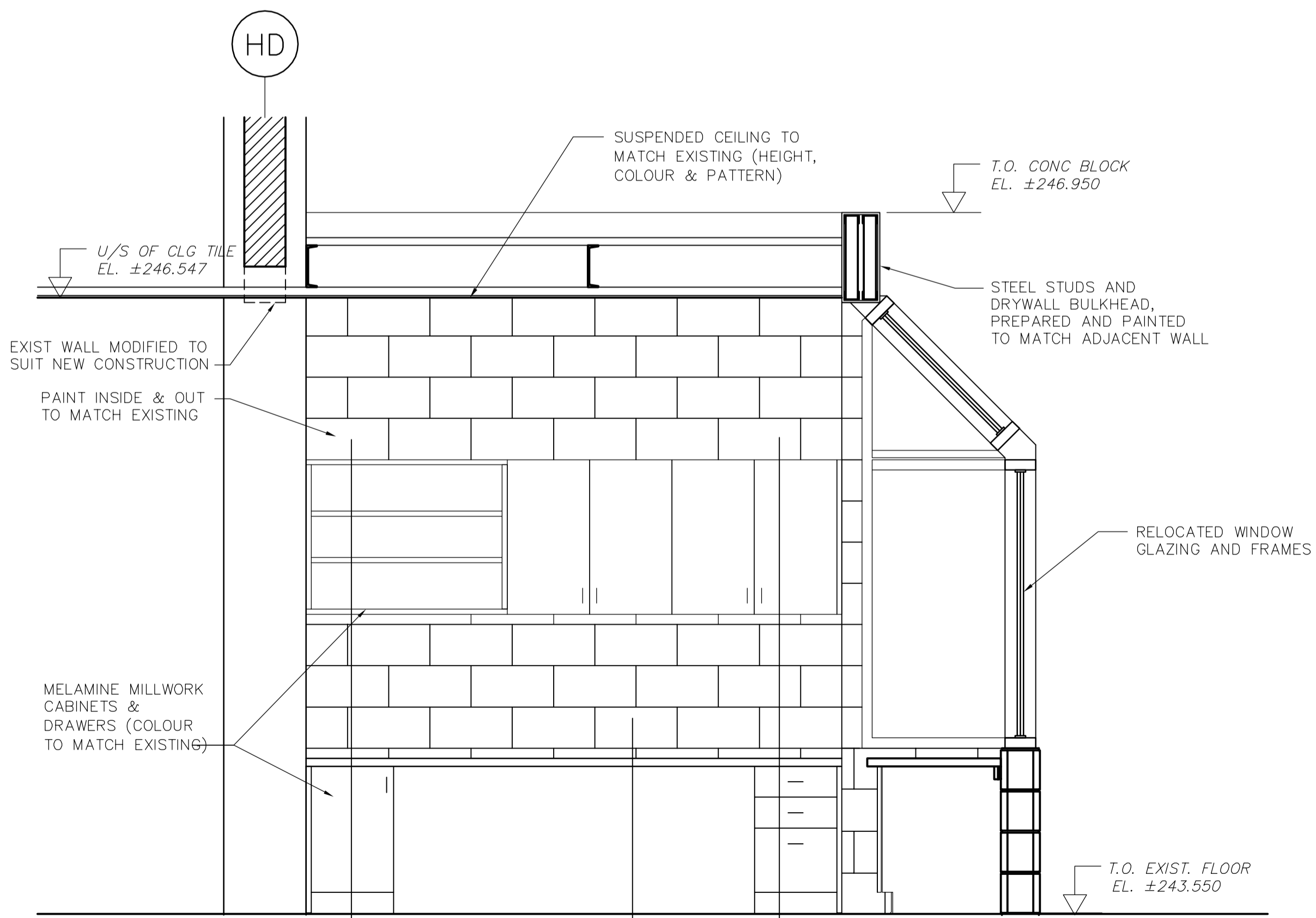
3 ENLARGED SECTION A1.01 1:20
