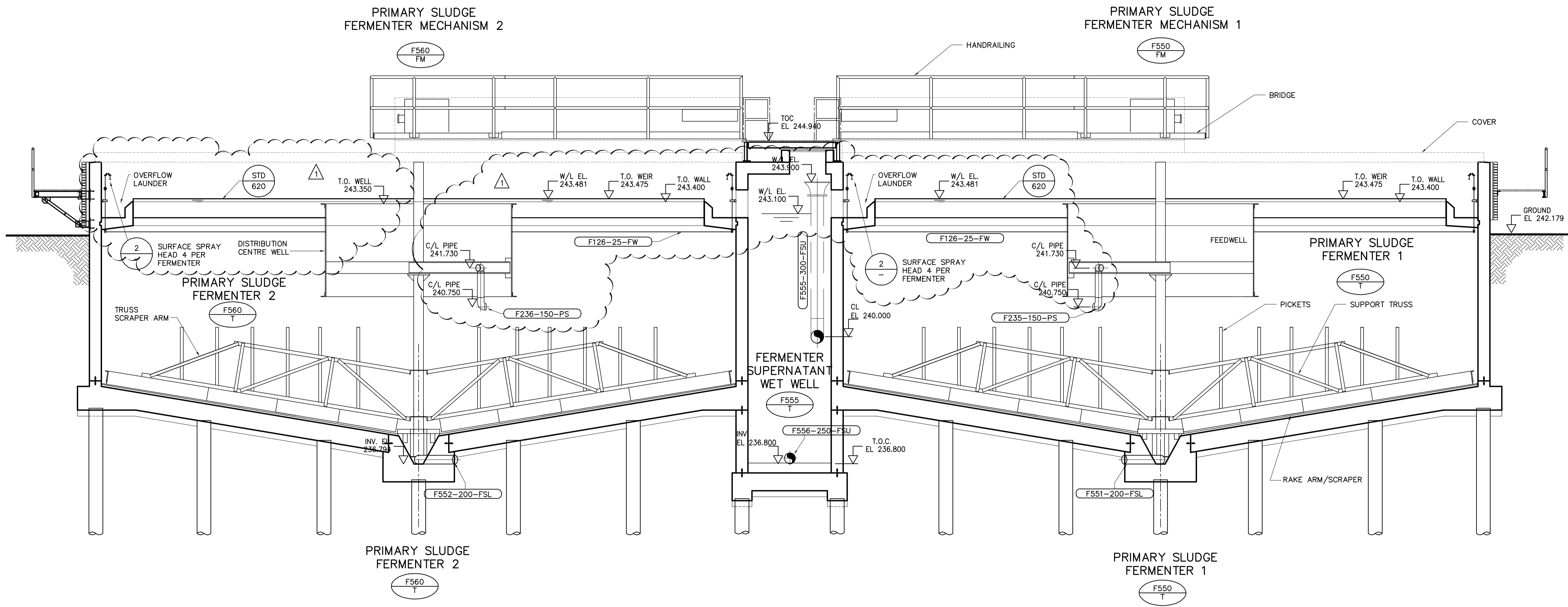
1 SECTION - PRIMARY SLUDGE FERMENTERS FP1.01 1:50
