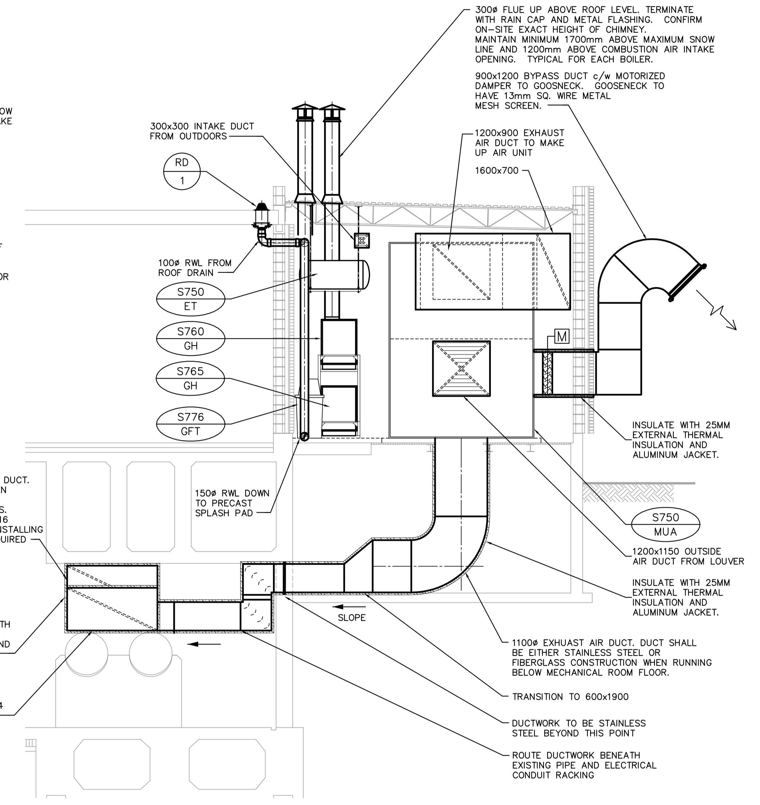
2 SECTION - MECHANICAL ROOM SM3.02 SCALE 1:50
