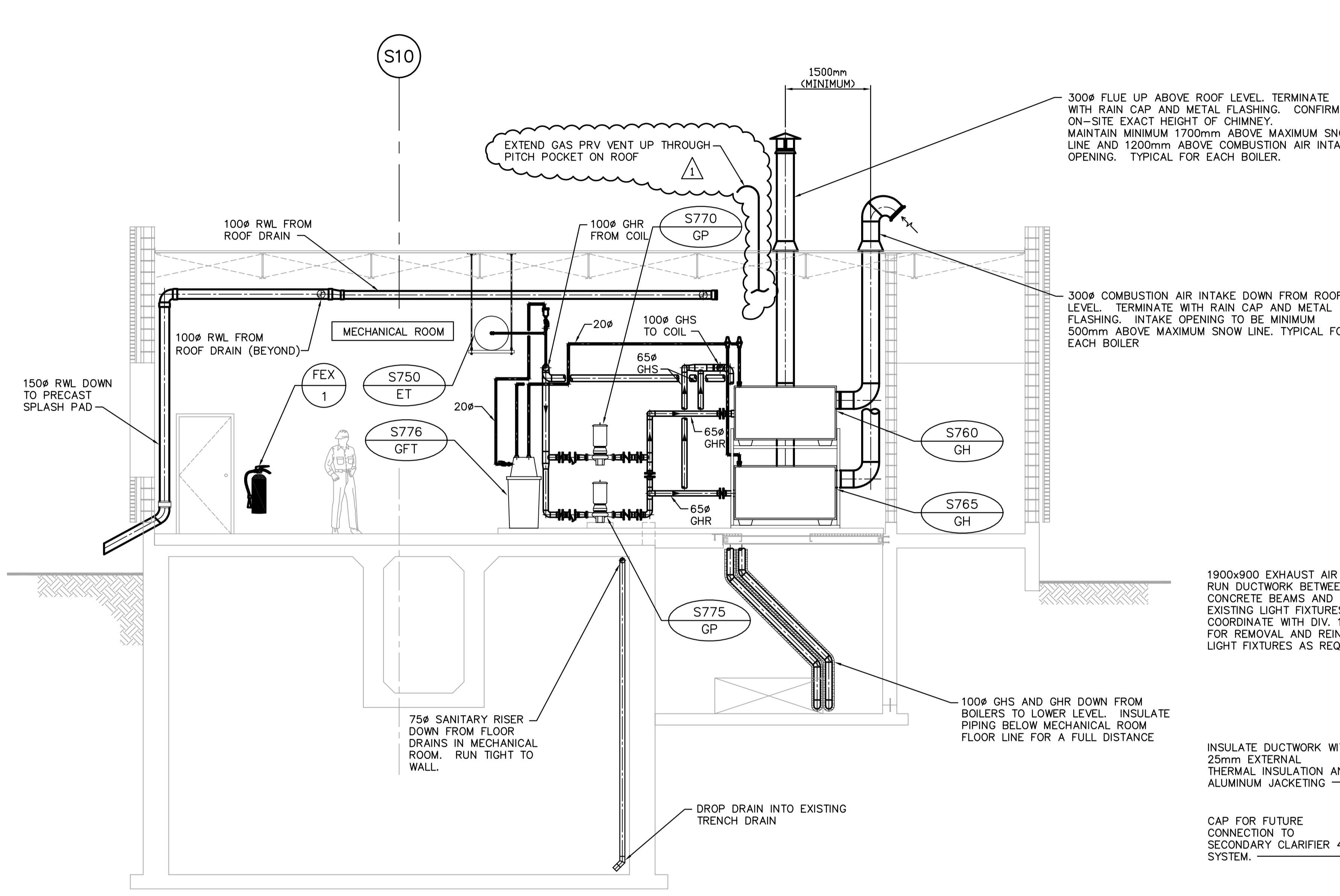
1 SECTION - MECHANICAL ROOM SM4.02 SCALE 1:50
