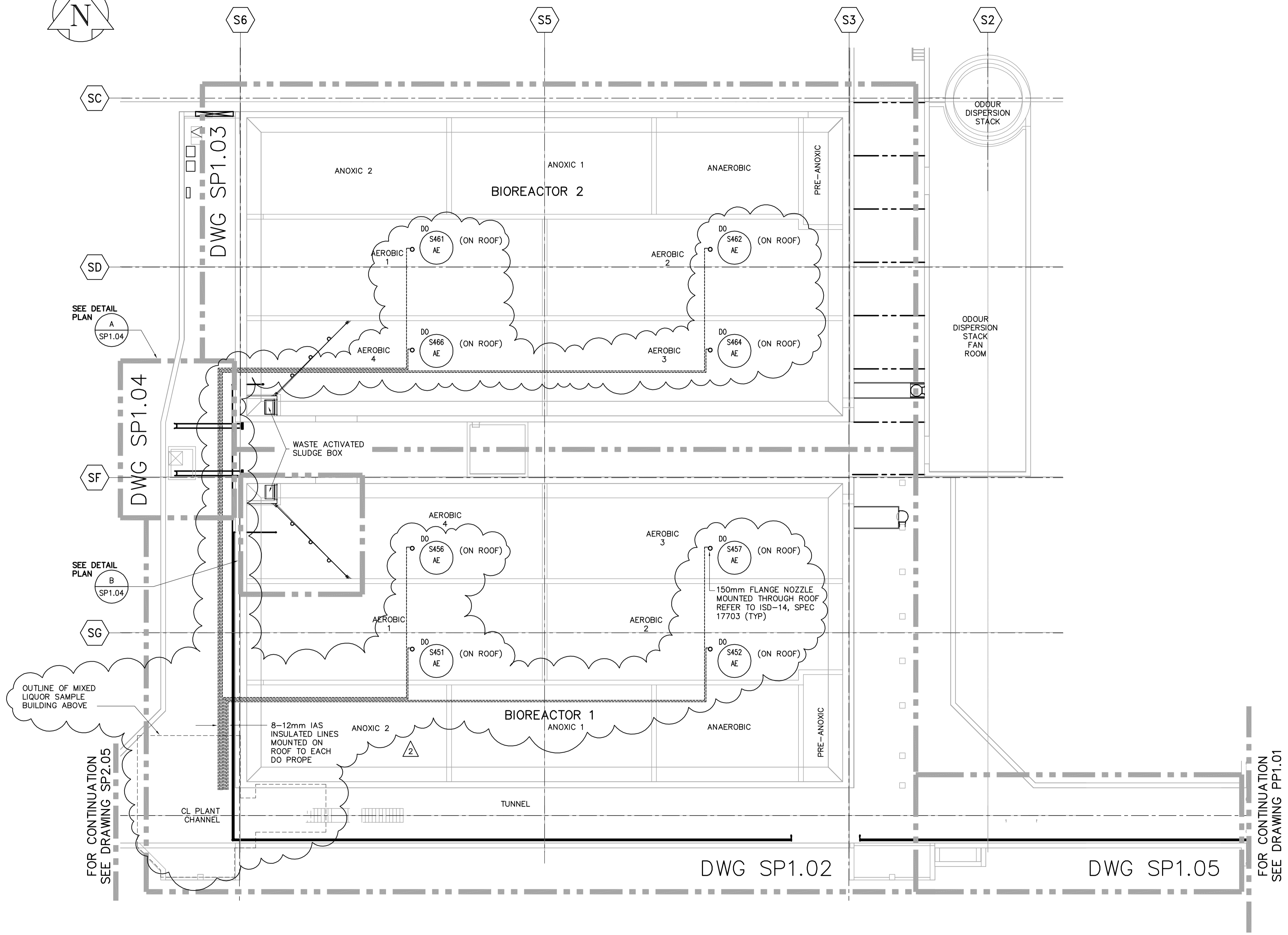
BIOREACTOR 1 AND 2 - PLAN 1:150
