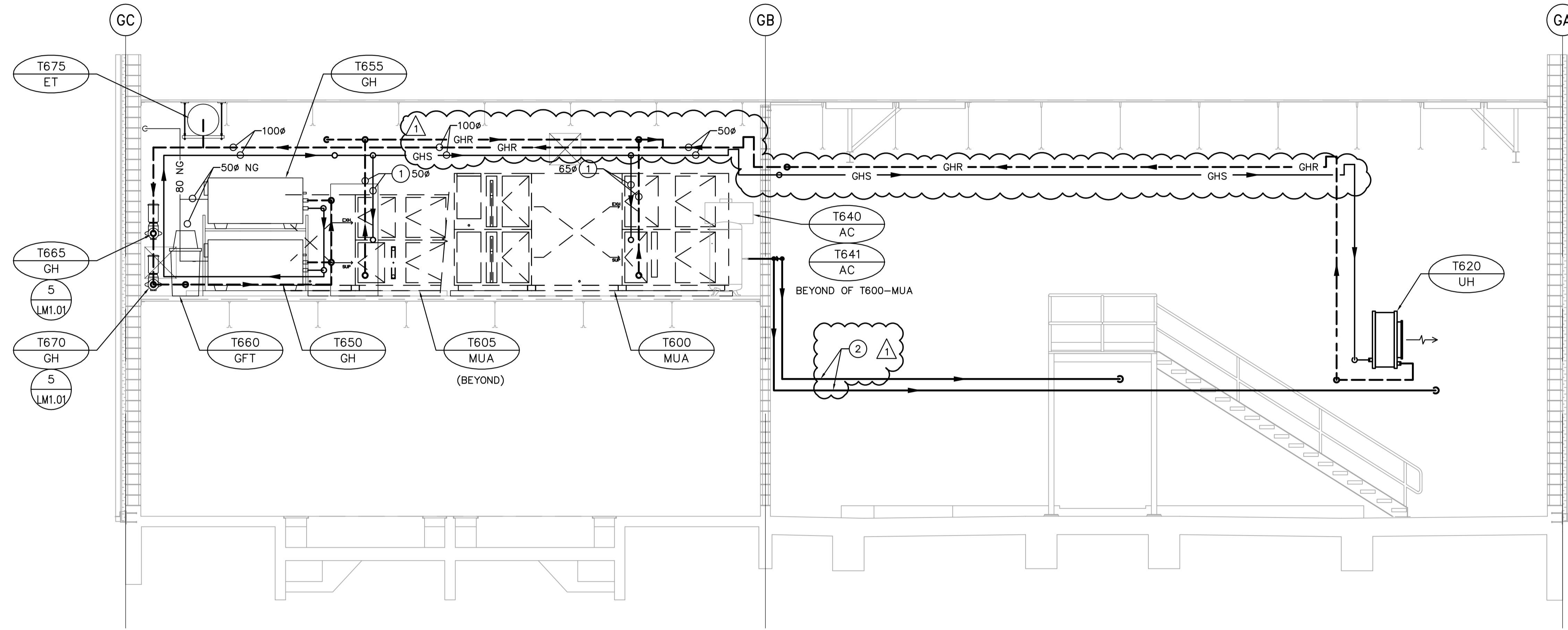
1 SECTION TM3.01 SCALE 1:50
