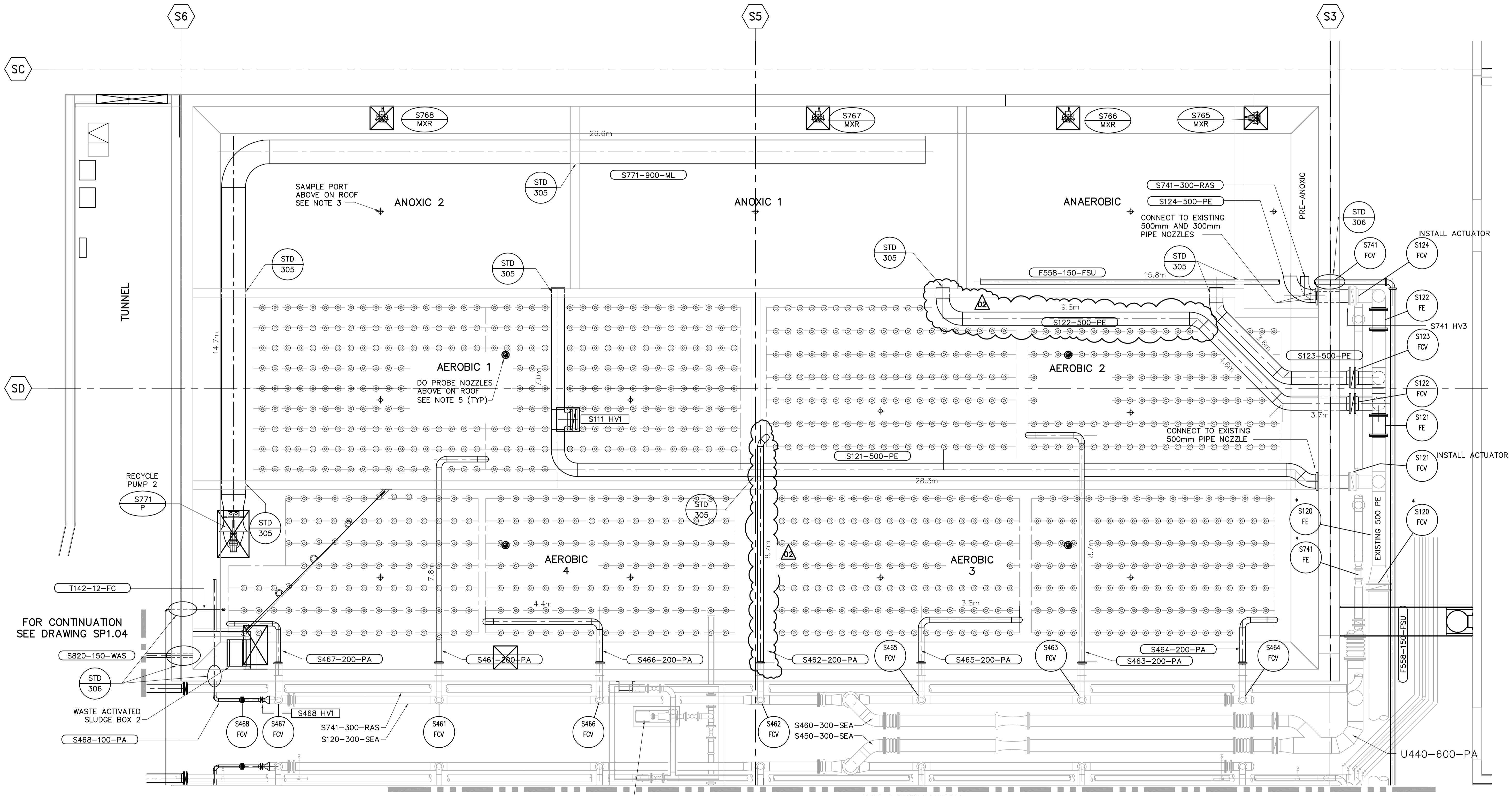
BIOREACTOR 2 - PLAN 1:75
