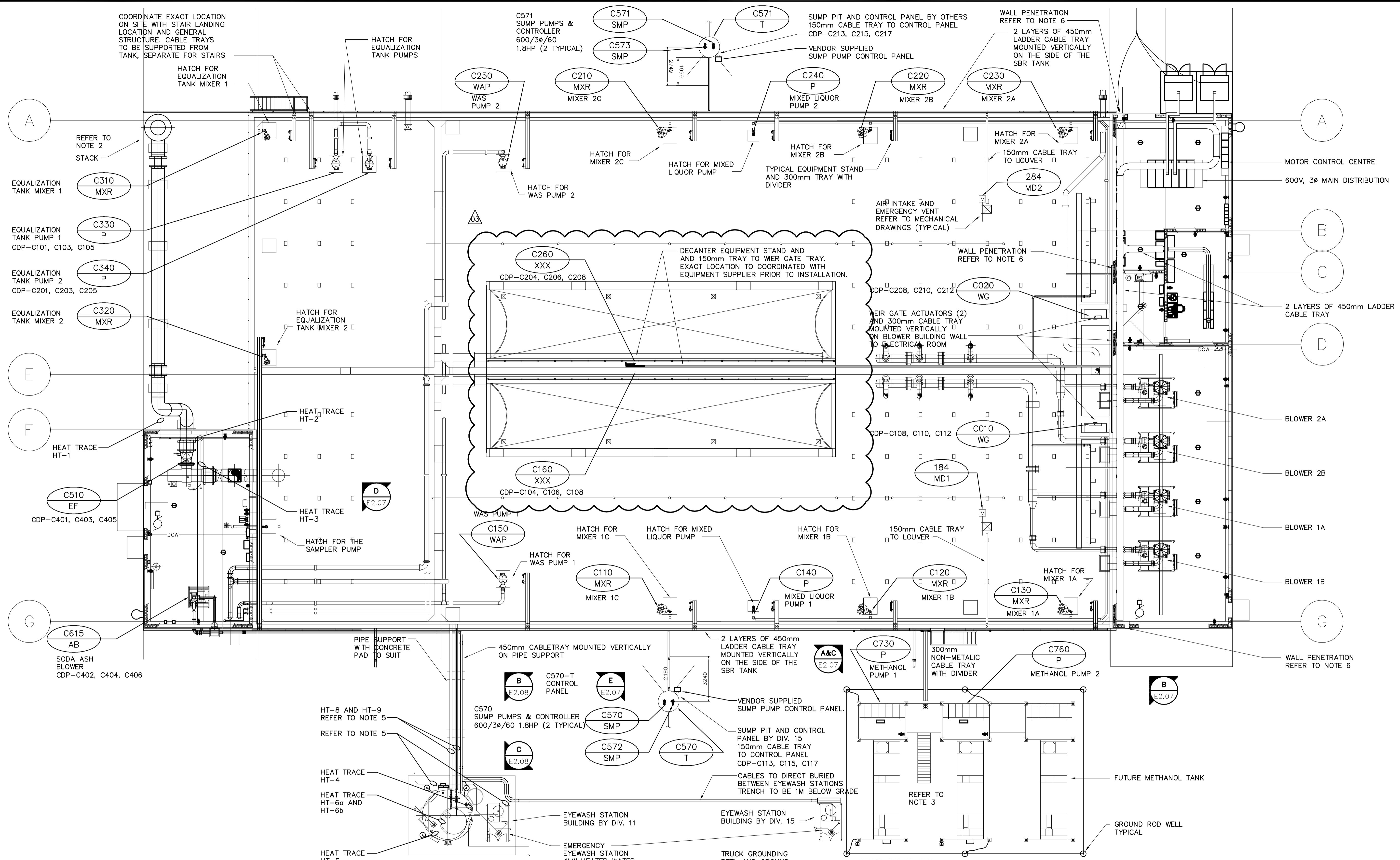
1 DETAIL - SBR BASIN AND EQUALIZATION TANKS PLAN E2.05 SCALE: N.T.S.
