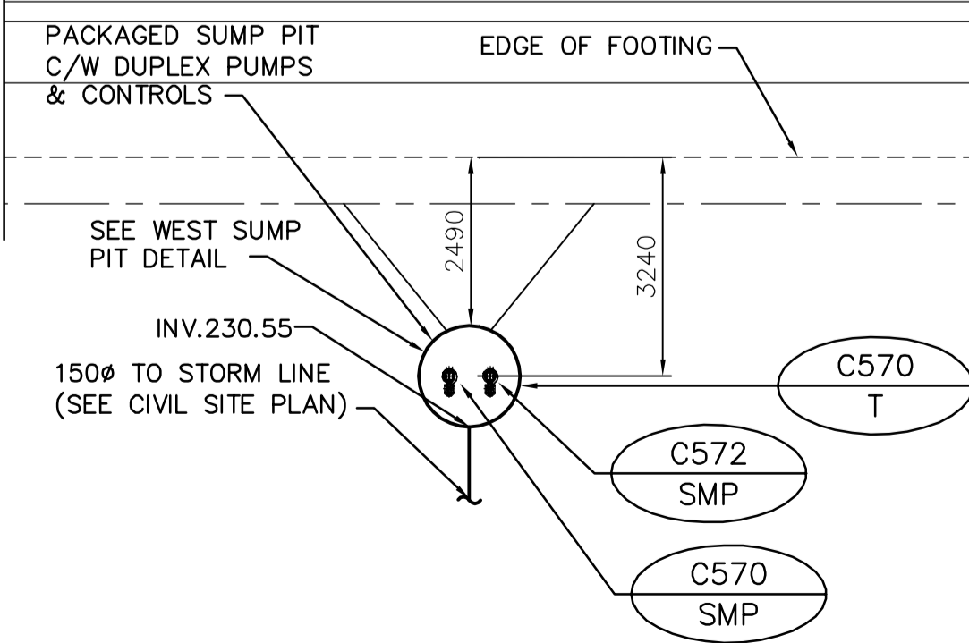
1 PARTIAL SBR BUILDING PLAN M1.03 SCALE 1:100
