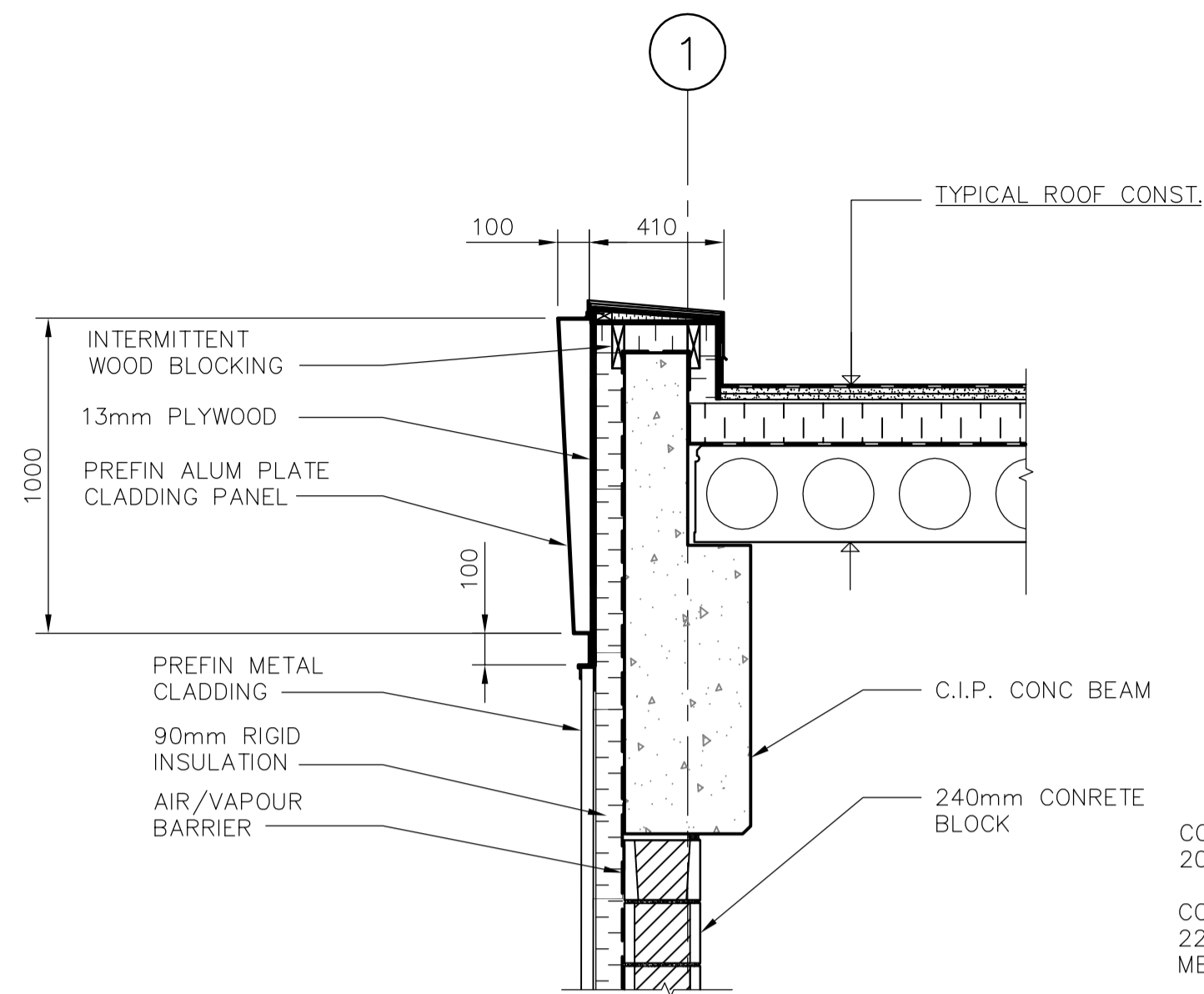
4 ROOF/WALL SECTION DETAIL WG-B0202 1:20
