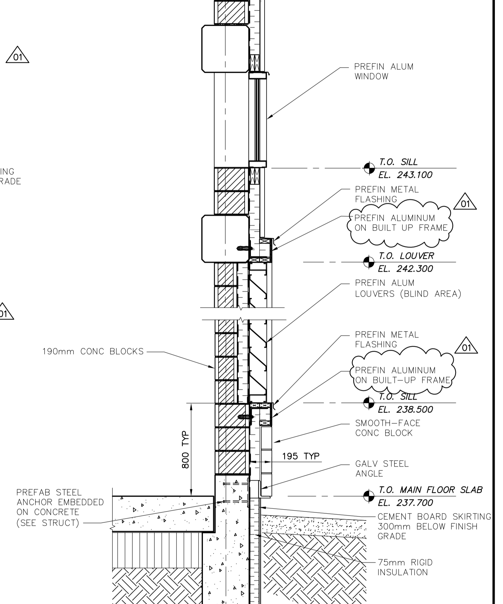
7 WALL SECTION DETAIL WG-B0203 1:20
