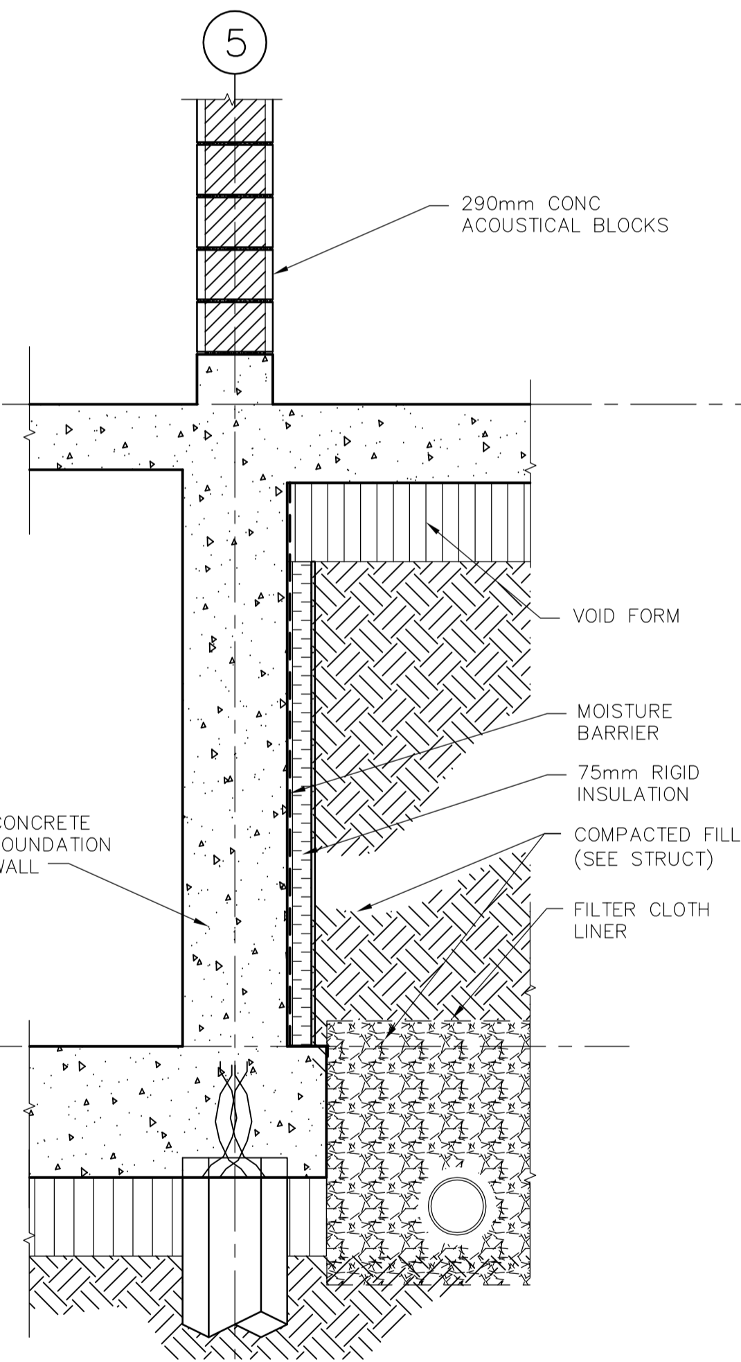
2 FOUNDATION WALL SECTION DETAIL WG-B0202 1:20
