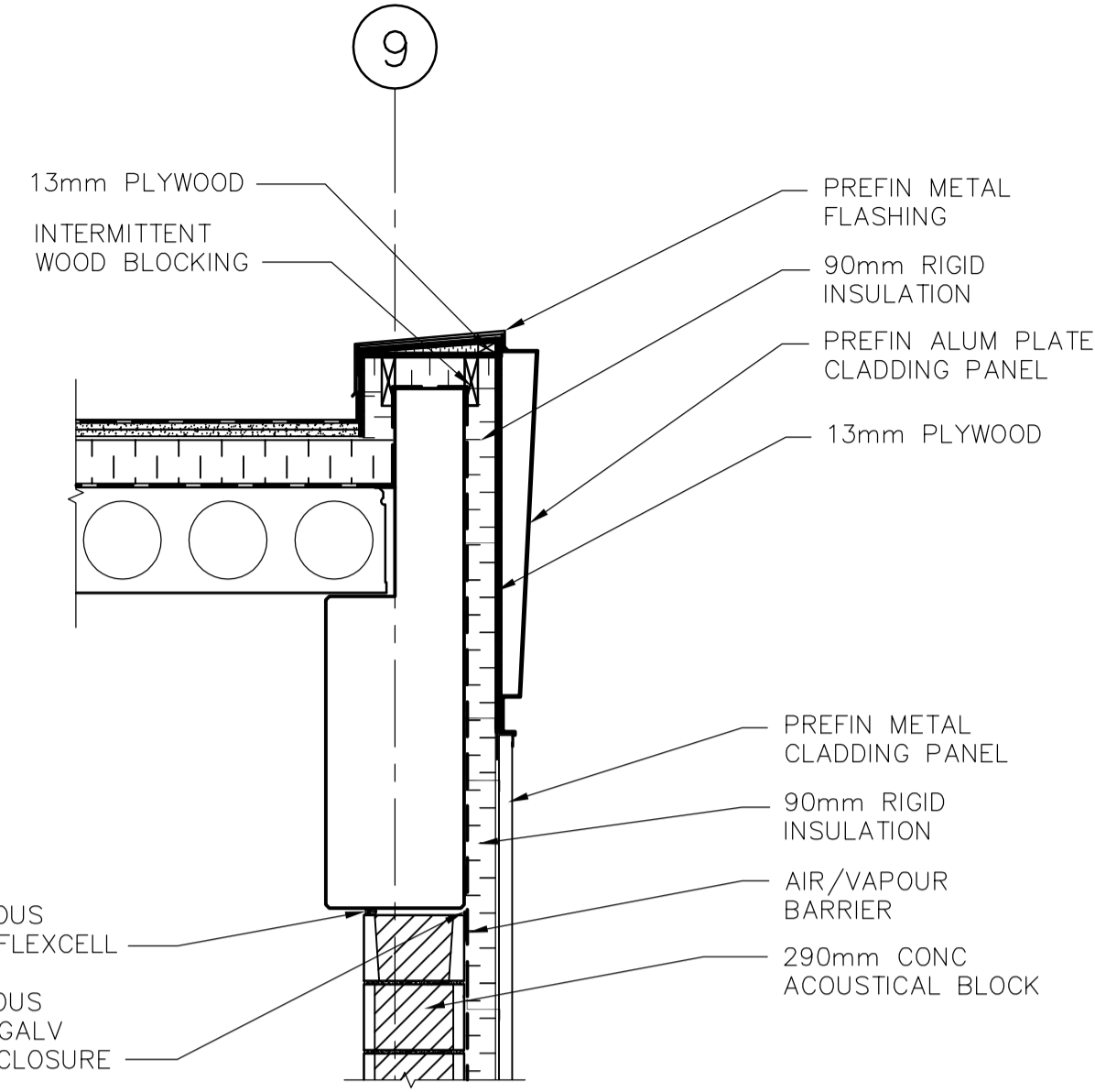
5 ROOF/WALL SECTION DETAIL WG-B0202 1:20
