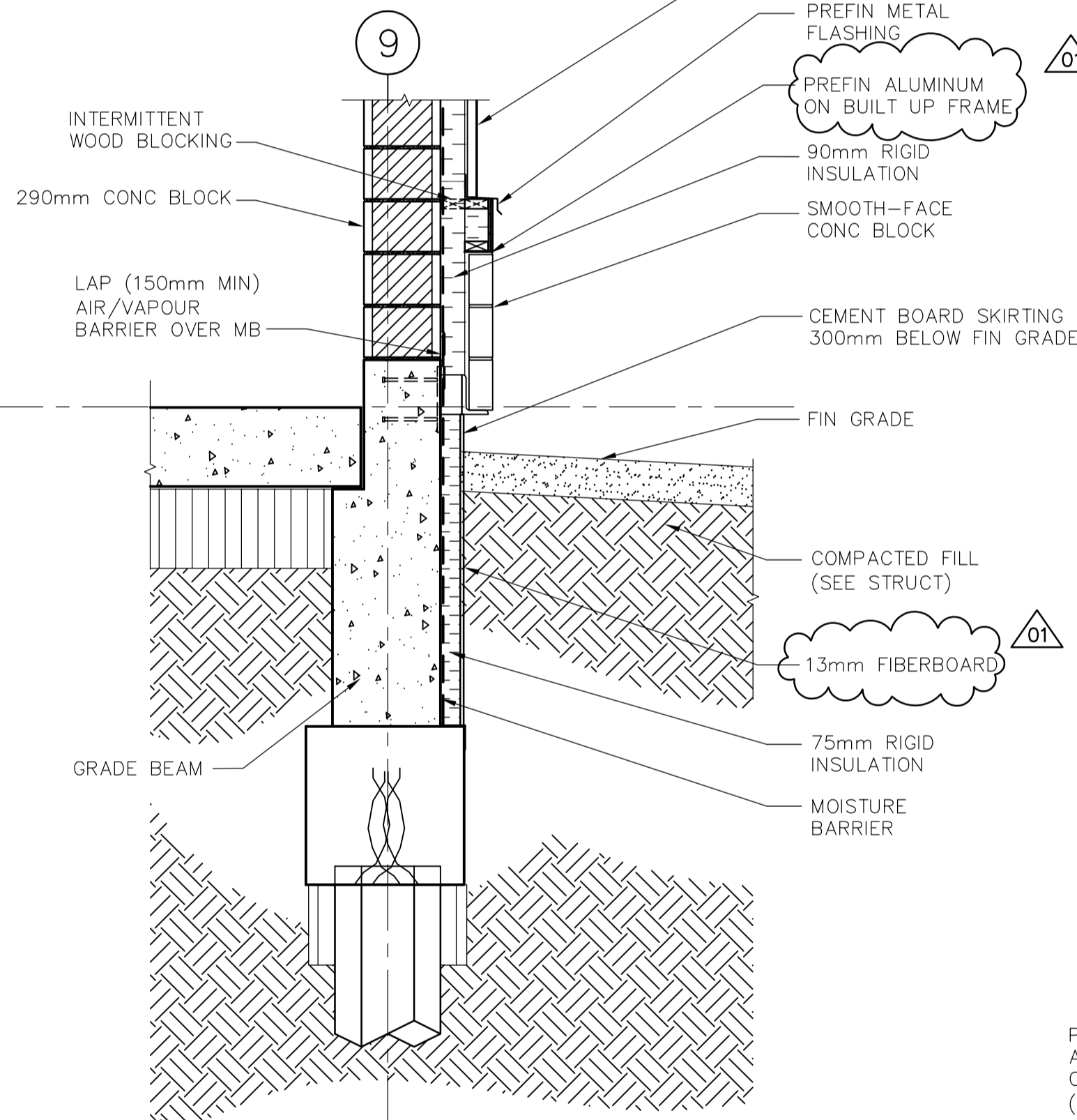
3 FOUNDATION WALL SECTION DETAIL WG-B0202 1:20
