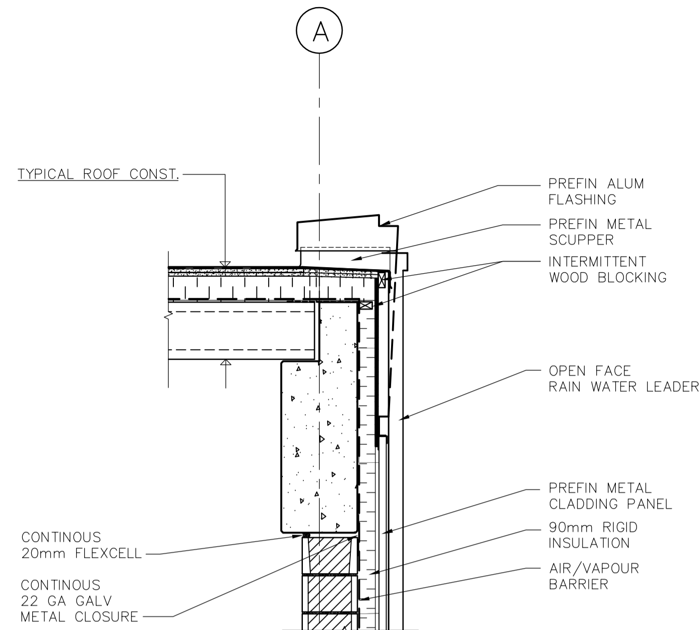
6 SCUPPER DETAIL WG-B0140 1:20
