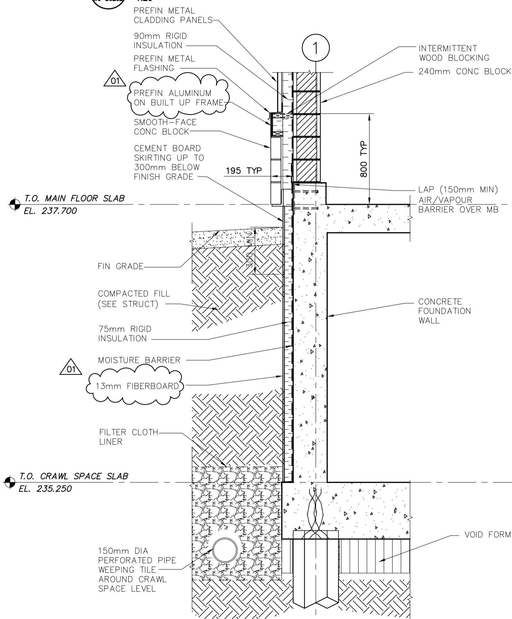
1 FOUNDATION WALL SECTION DETAIL WG-B0202 1:20
