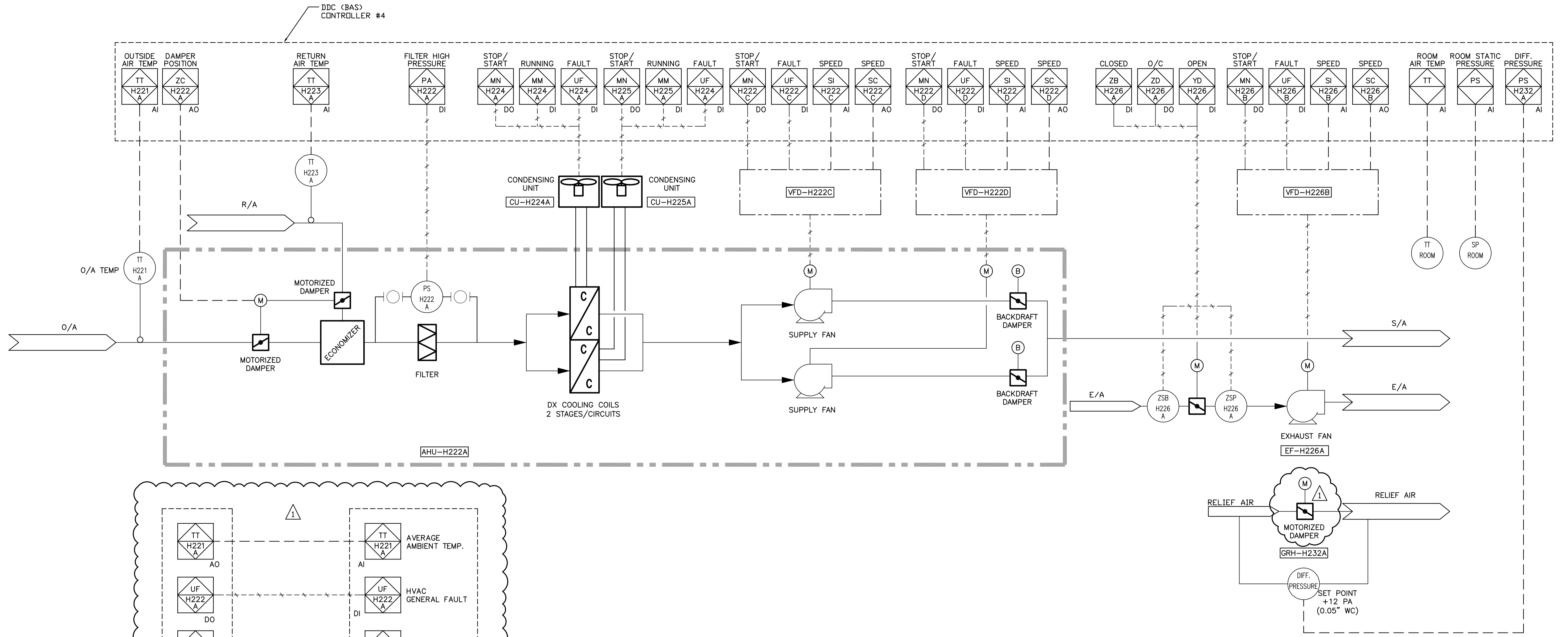
1 ELECTRICAL ROOM COOLING AND VENTILATION UNIT AHU-H222A N.T.S.
