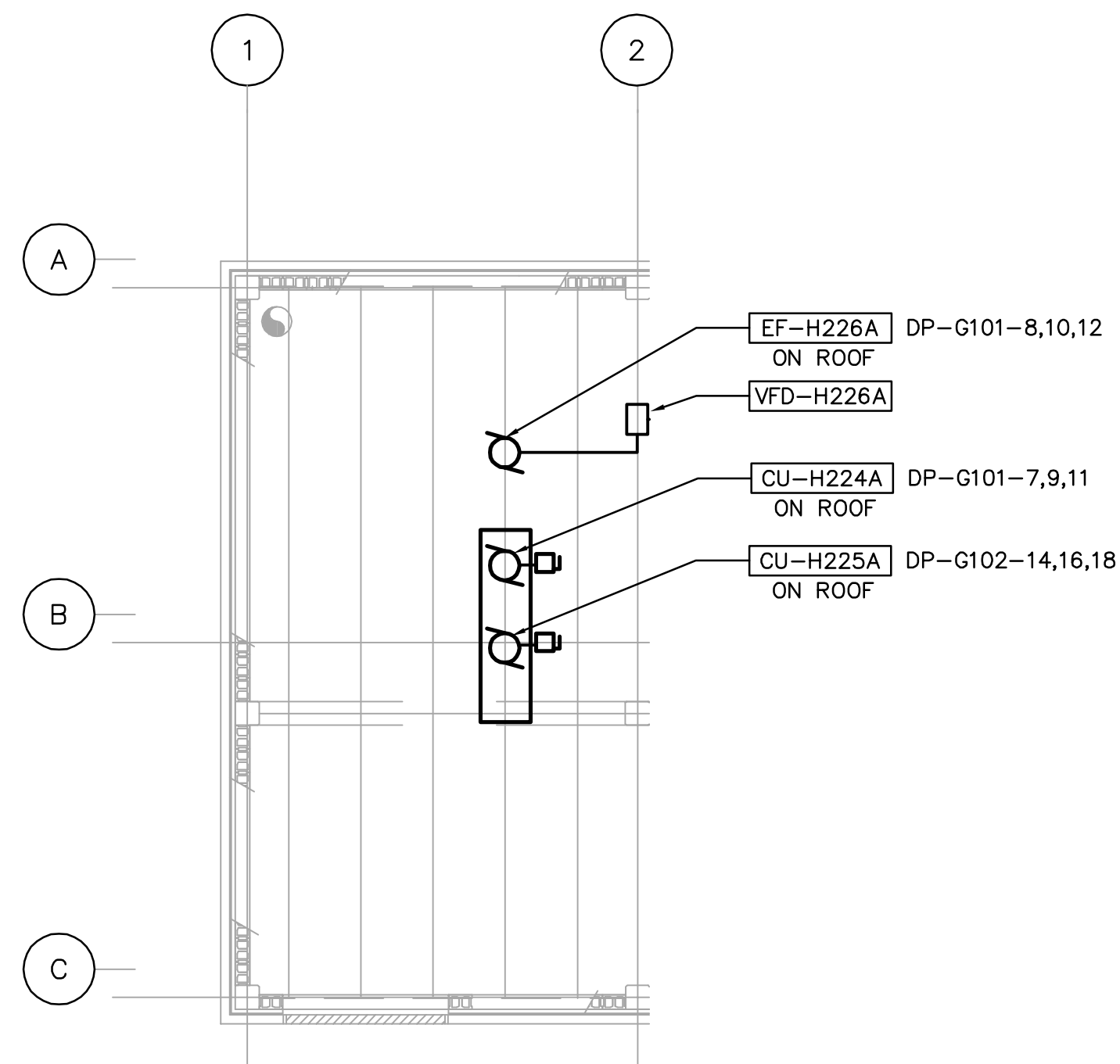
ROOF POWER PLAN 1:100
