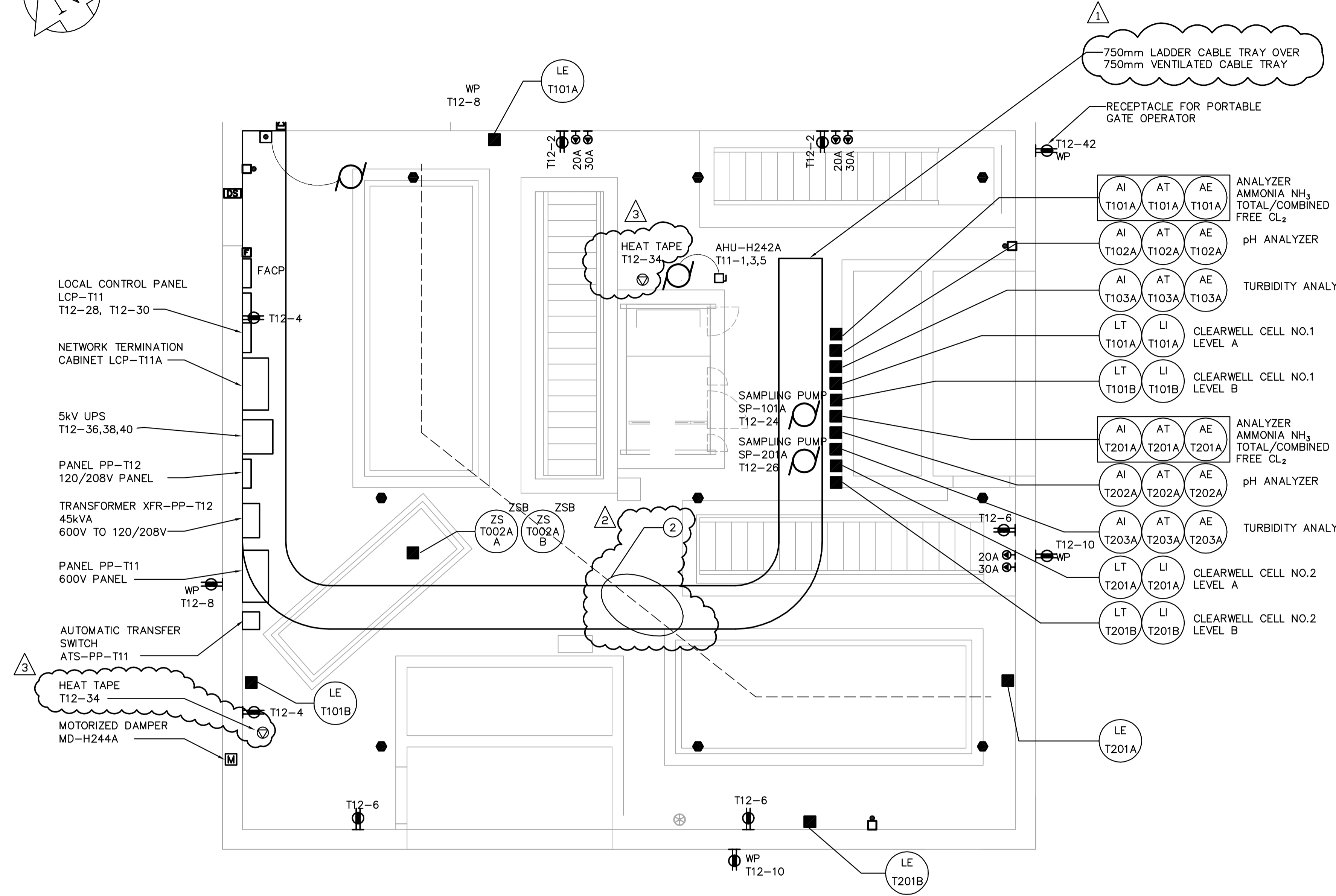
INLET BUILDING MAIN FLOOR POWER PLAN 1:50
