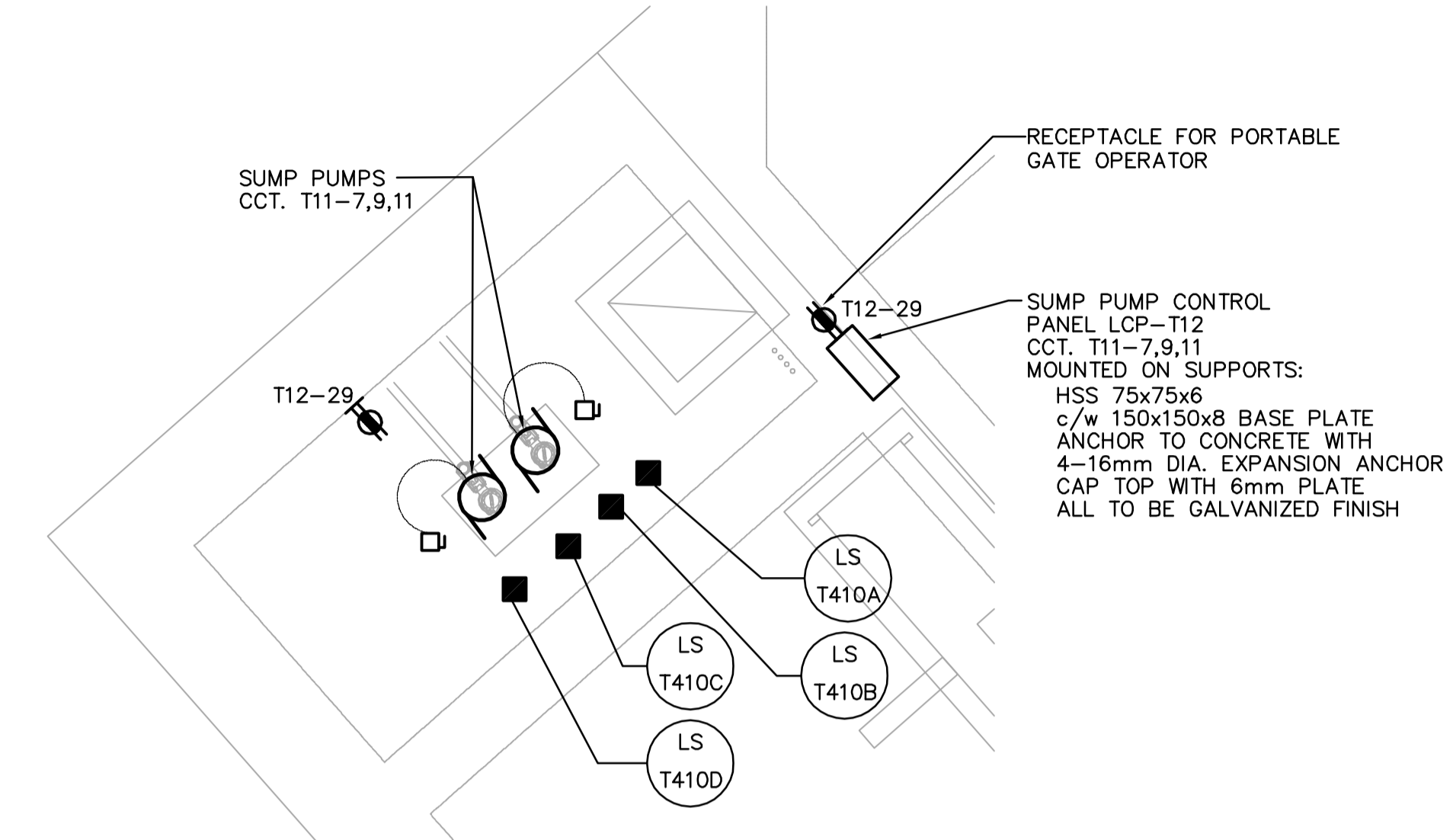
SUMP PIT AREA POWER PLAN 1:50
