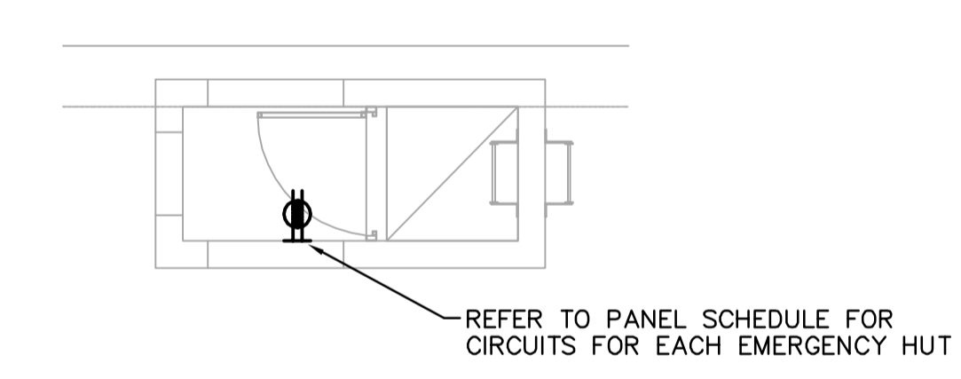
EMERGENCY HUT POWER PLAN 1:50
