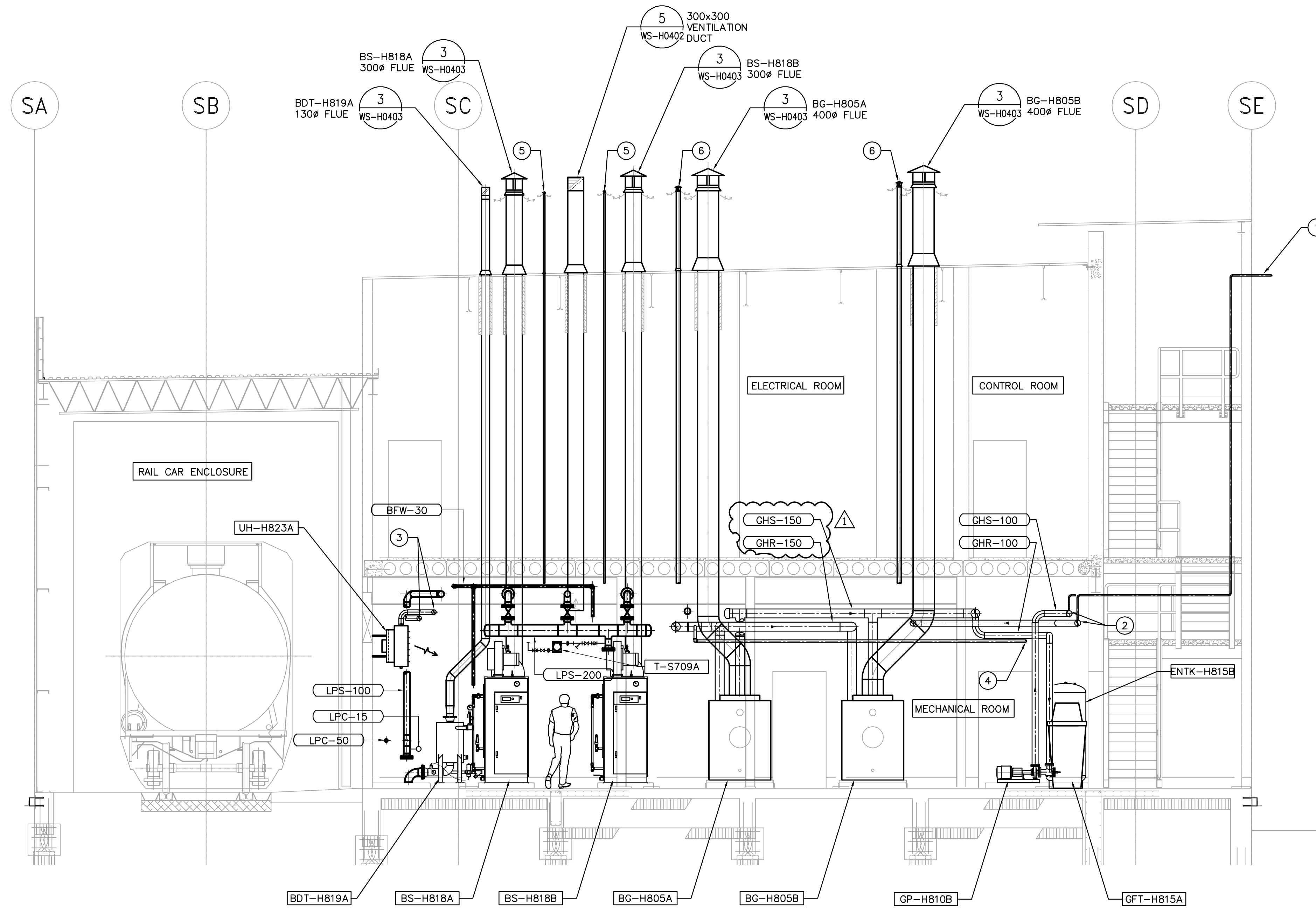
A SECTION WS-H0110 1:50
