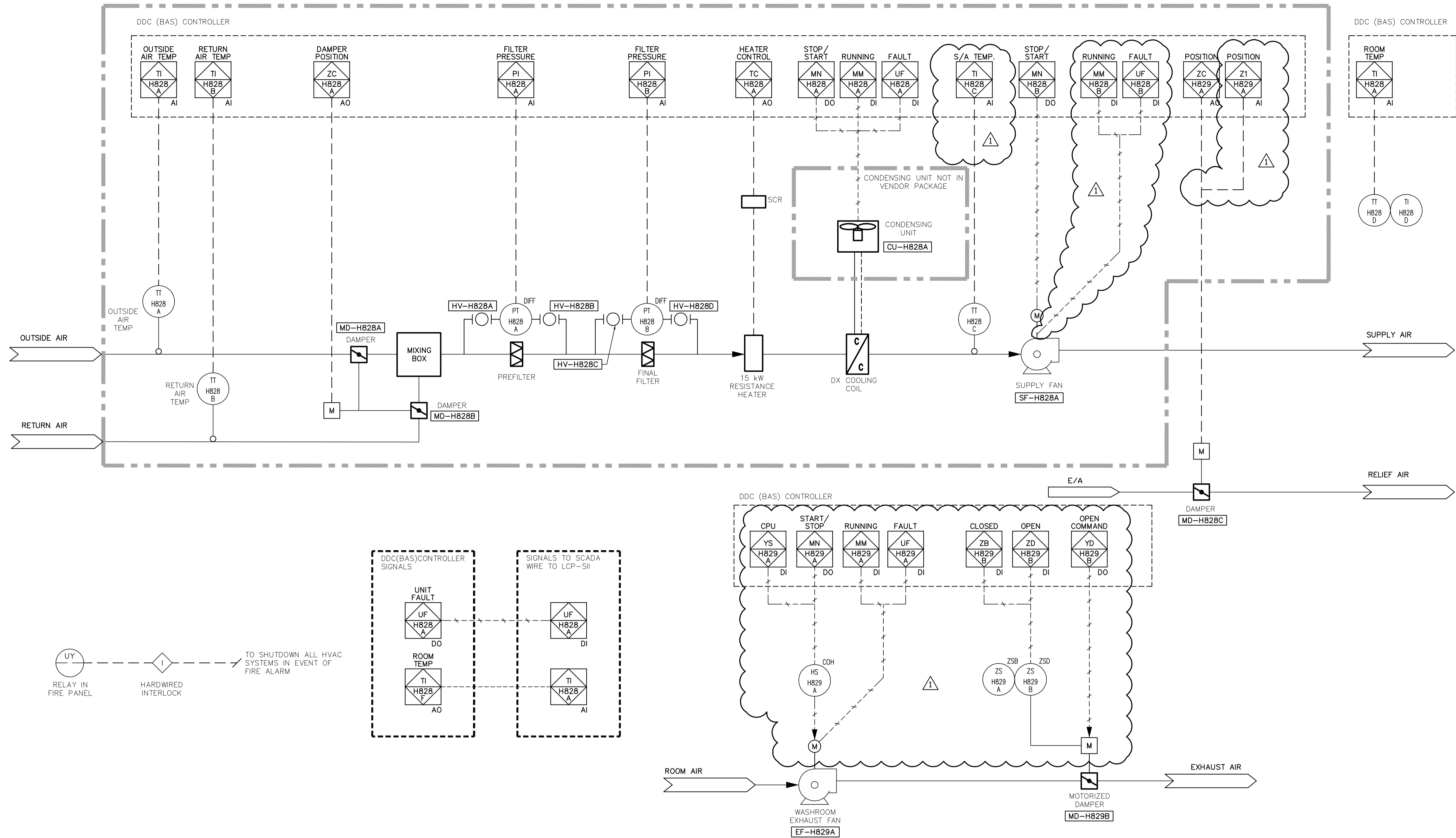
1 CONTROL ROOM HEATING, COOLING AND VENTILATION SCHEMATIC (AHU-H828A; EF-H829A) - N.T.S.
