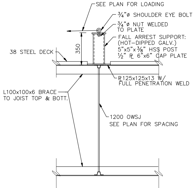
ROOF FALL ARREST DETAIL 1:20
