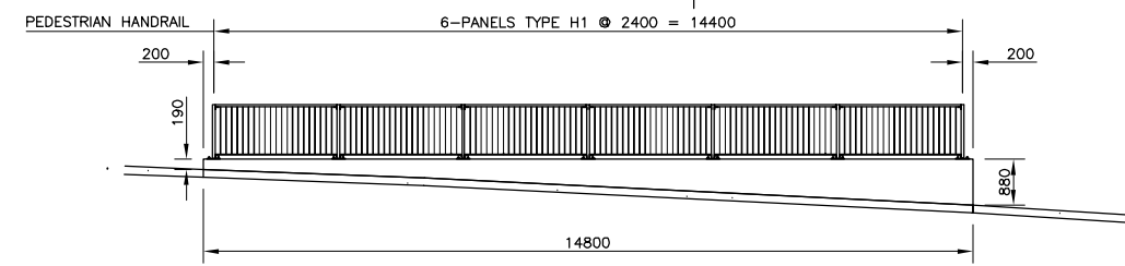
SOUTH SIDE OF CPR BRIDGE AT SOUTH EAST CORNER OF EXISTING BUILDING SIDEWALK RETAINING WALL ELEVATION 1: 75 LOOKING WEST
