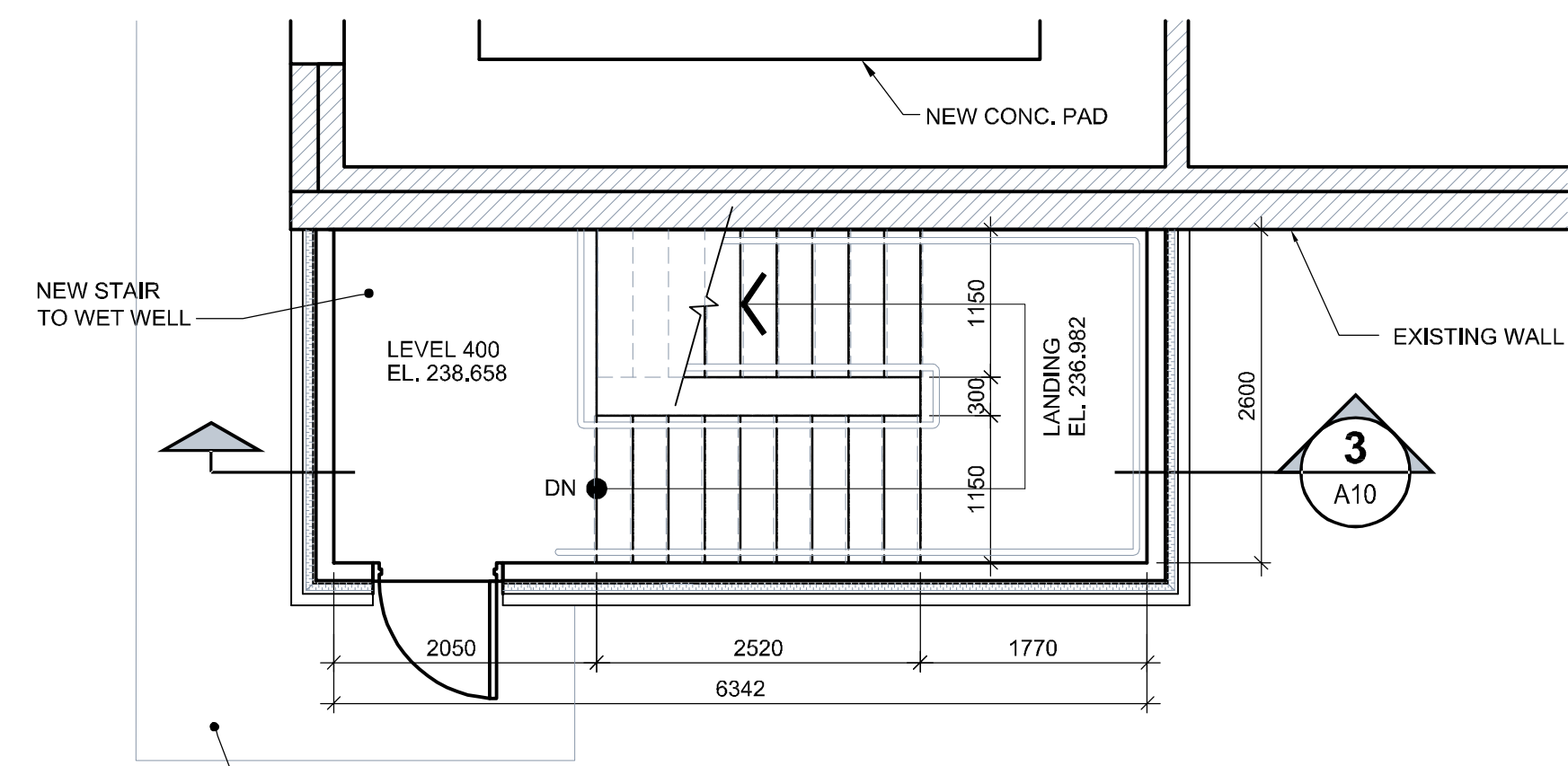
1 STAIR PLAN @ LEVEL 400 SCALE: 1:50
