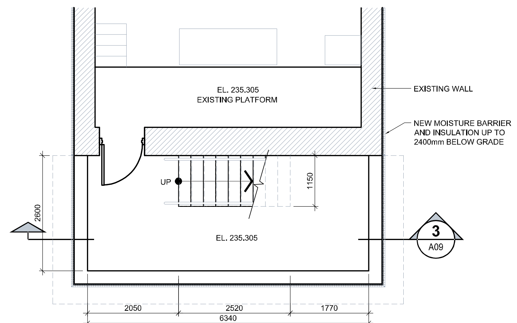
2 STAIR PLAN @ LEVEL 300 SCALE: 1:50
