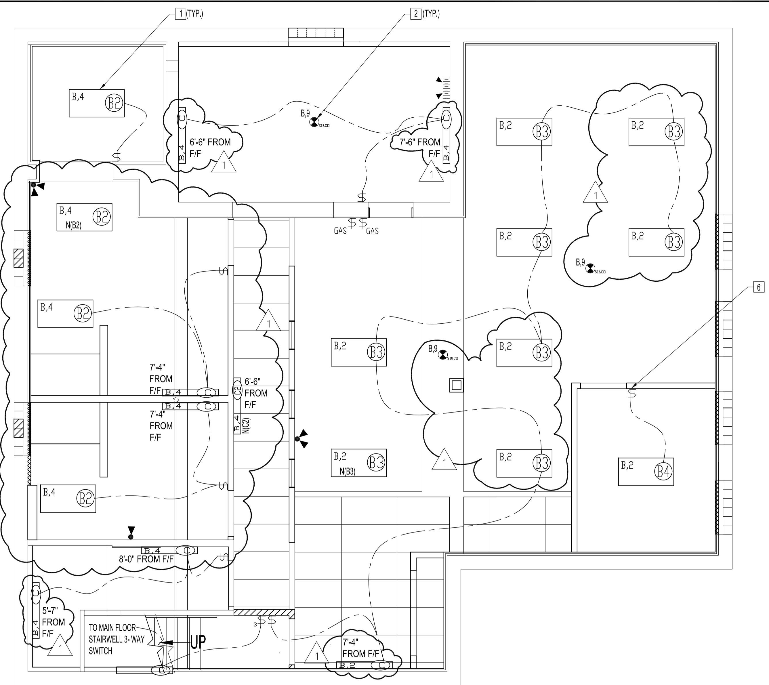
BASEMENT FLOOR PLAN - ELECTRICAL LIGHTING SCALE: 1/4"=1'-0"
