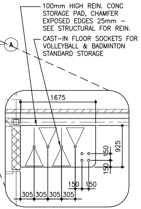
2 STOR. DETAIL DA-6 SCALE: 1:50 NEW DRAWING
