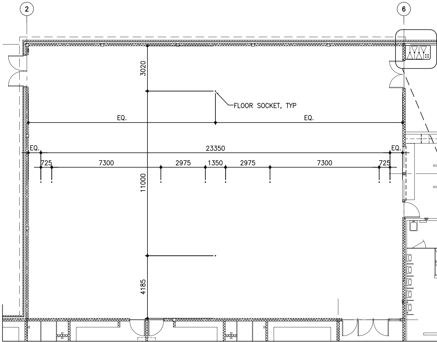
1 COMPLETE FLOOR SOCKET LAYOUT DA-6 SCALE: 1:150 NEW DRAWING
