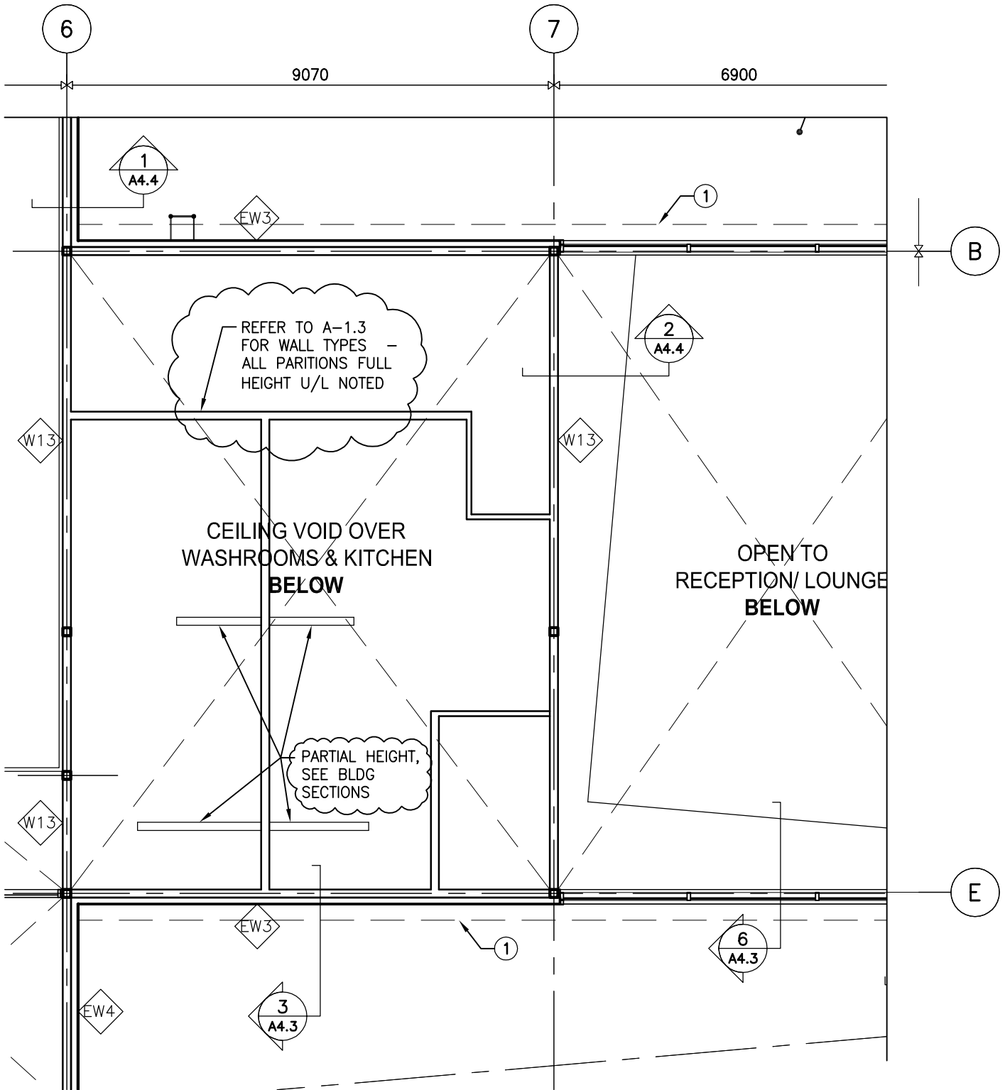
1 MEZZ. FLOOR PLAN A-1.4 SCALE: 1:100 REVISED DRAWING
