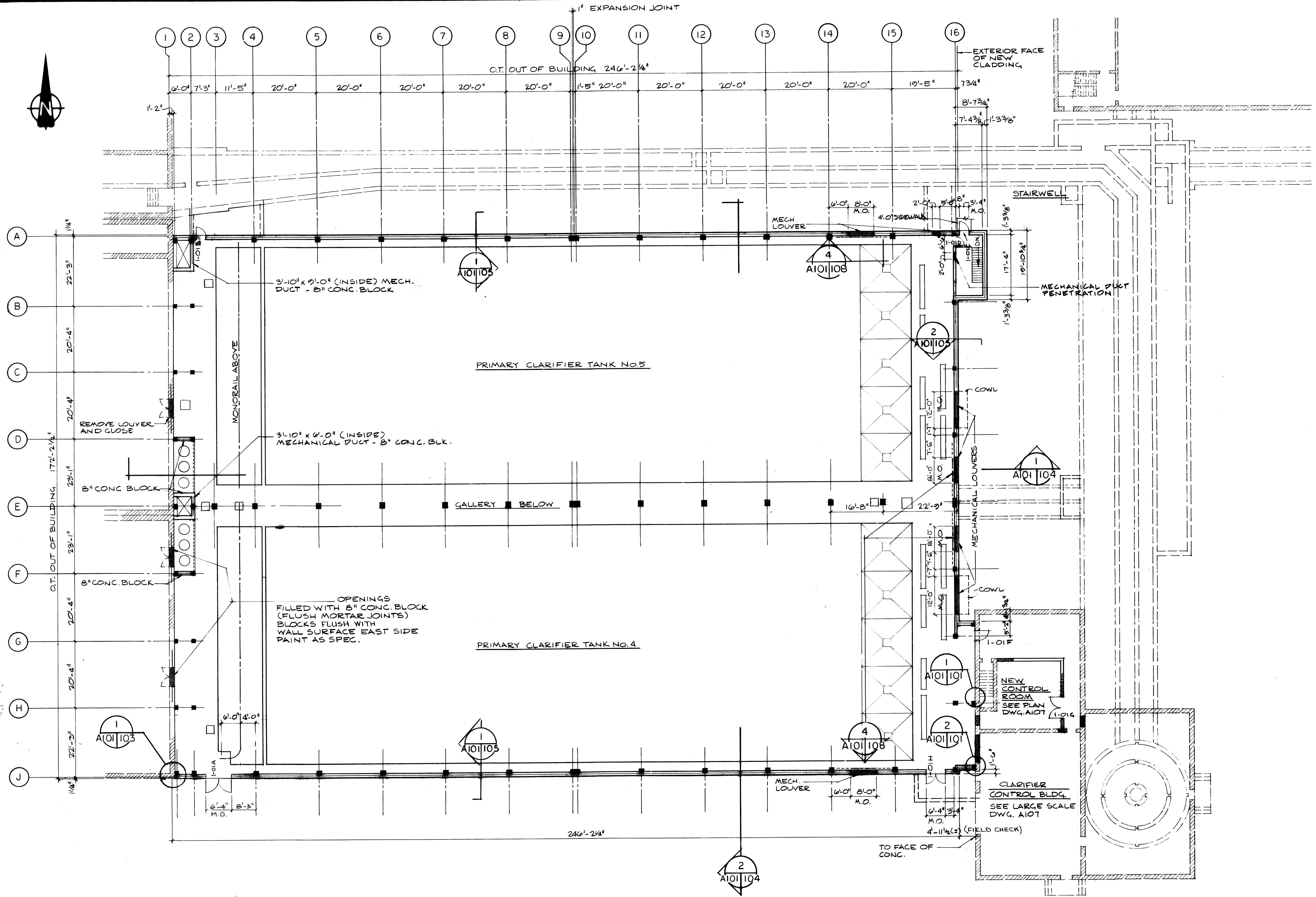
FLOOR PLAN AT EL. 33.50' 1/16" = 1'-0"
