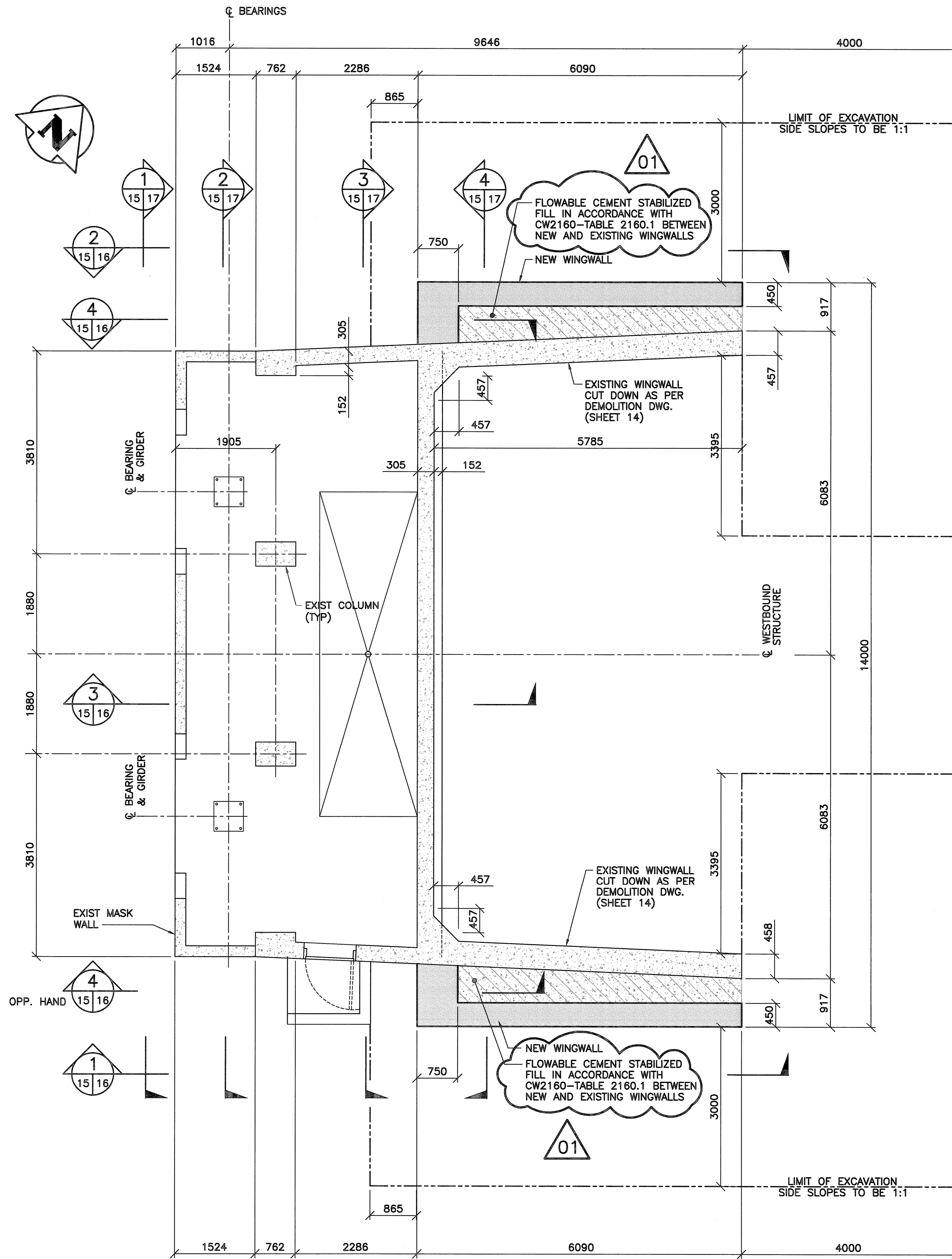
1 LOWER LEVEL PLAN 1 : 50
