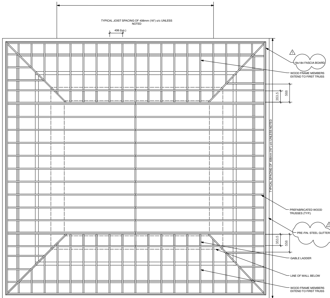
1 ROOF FRAMING PLAN A3 Scale: 1:25
