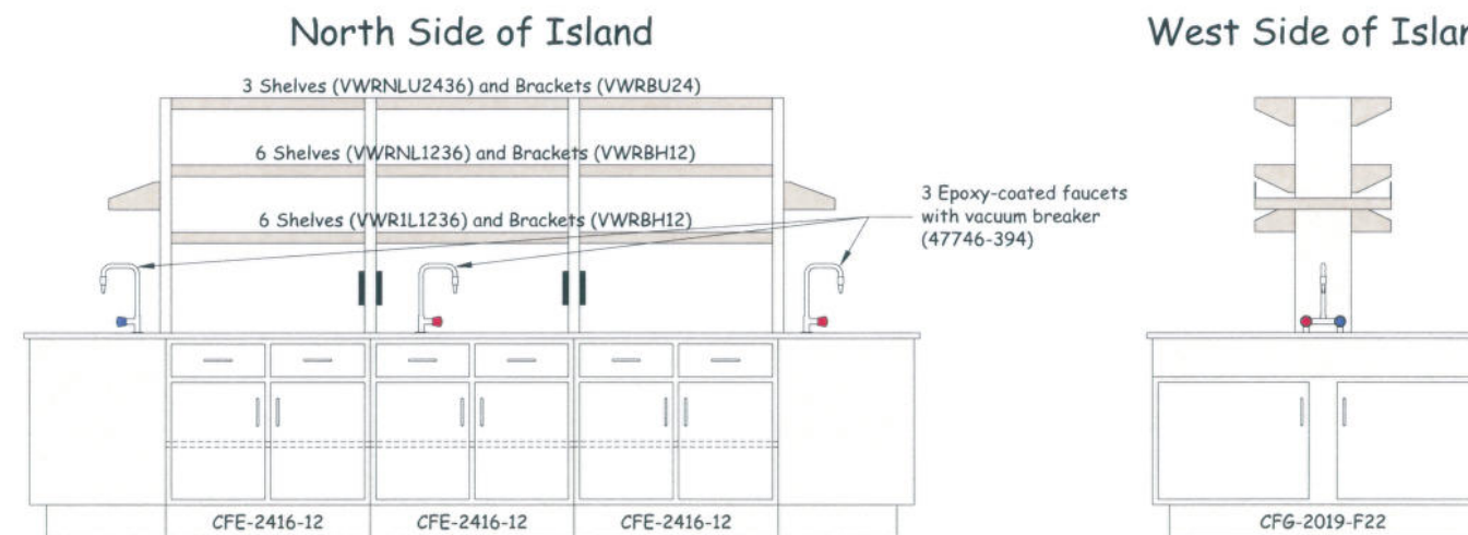
Drawing 02-R1
