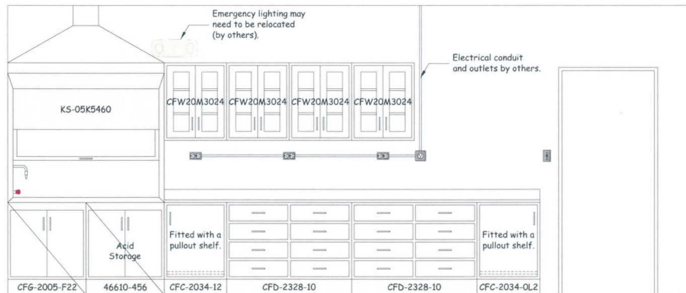
South Wall
