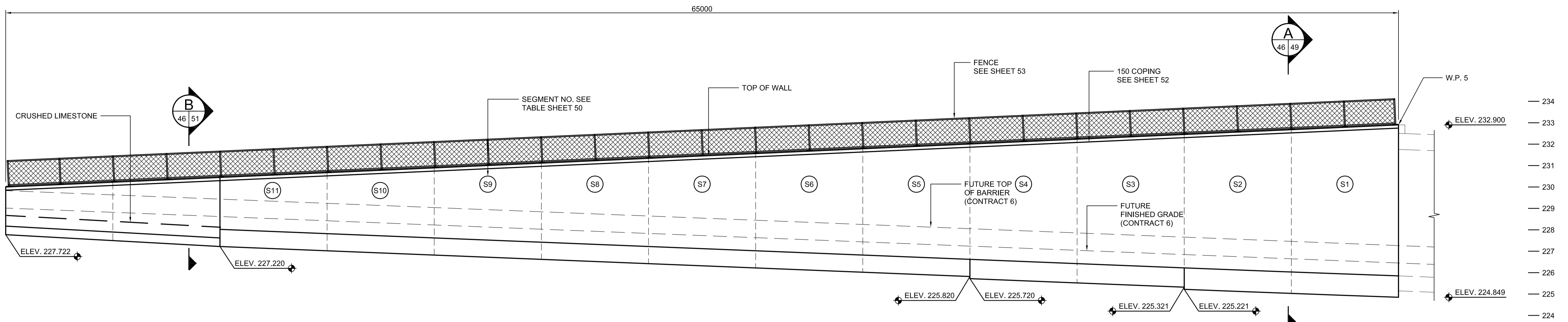
SOUTHWEST WALL ELEVATION SCALE 1:100
