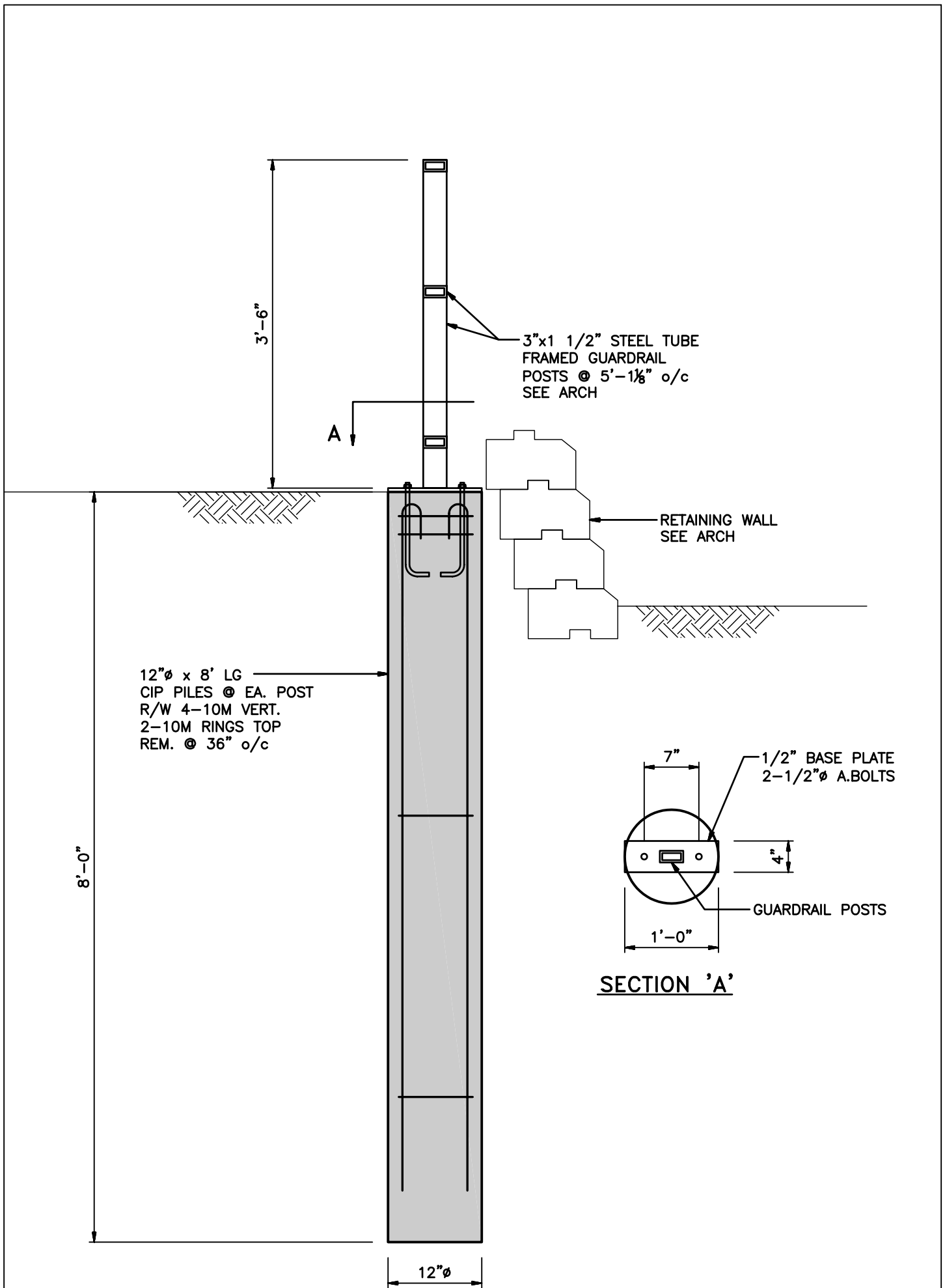
6 S-3 GUARDRAIL FOUNDATION 3/4" = 1'-0"
