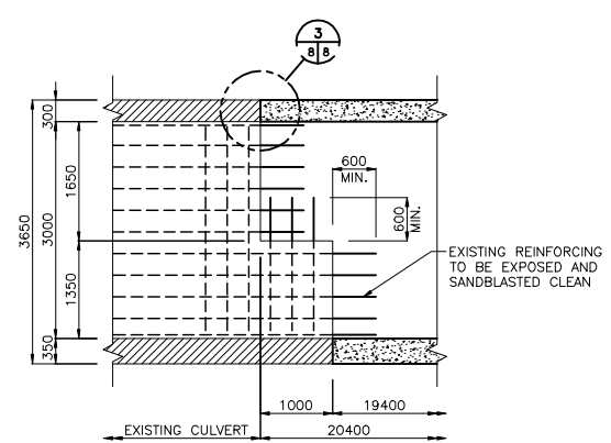
A 8 8 1:50 CULVERT SPLICE SECTION
