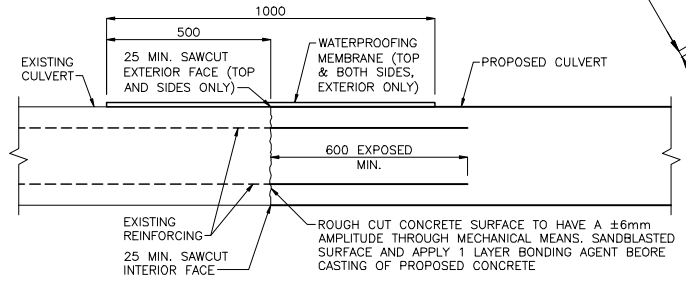
3 8 8 1:10 CULVERT SPLICE DETAIL
