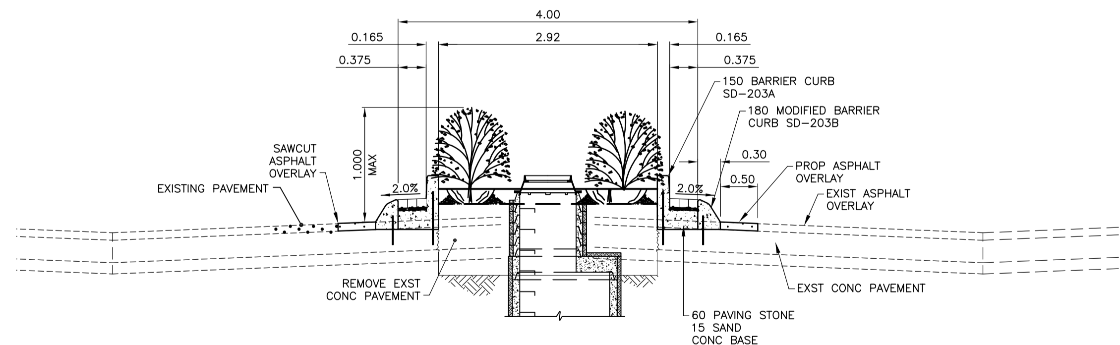
A KENNY STREET & EUGENIE STREET SECTION 1:50H 1:25V
