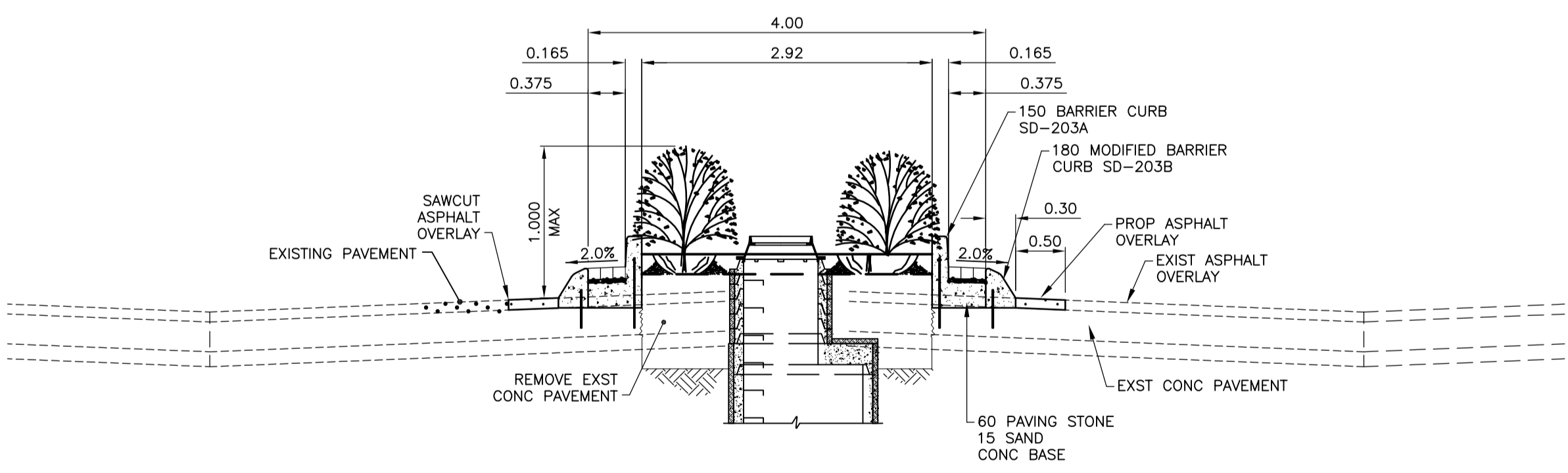
A BRAEMAR AVENUE & EUGENIE STREET SECTION 1:50H 1:25V
