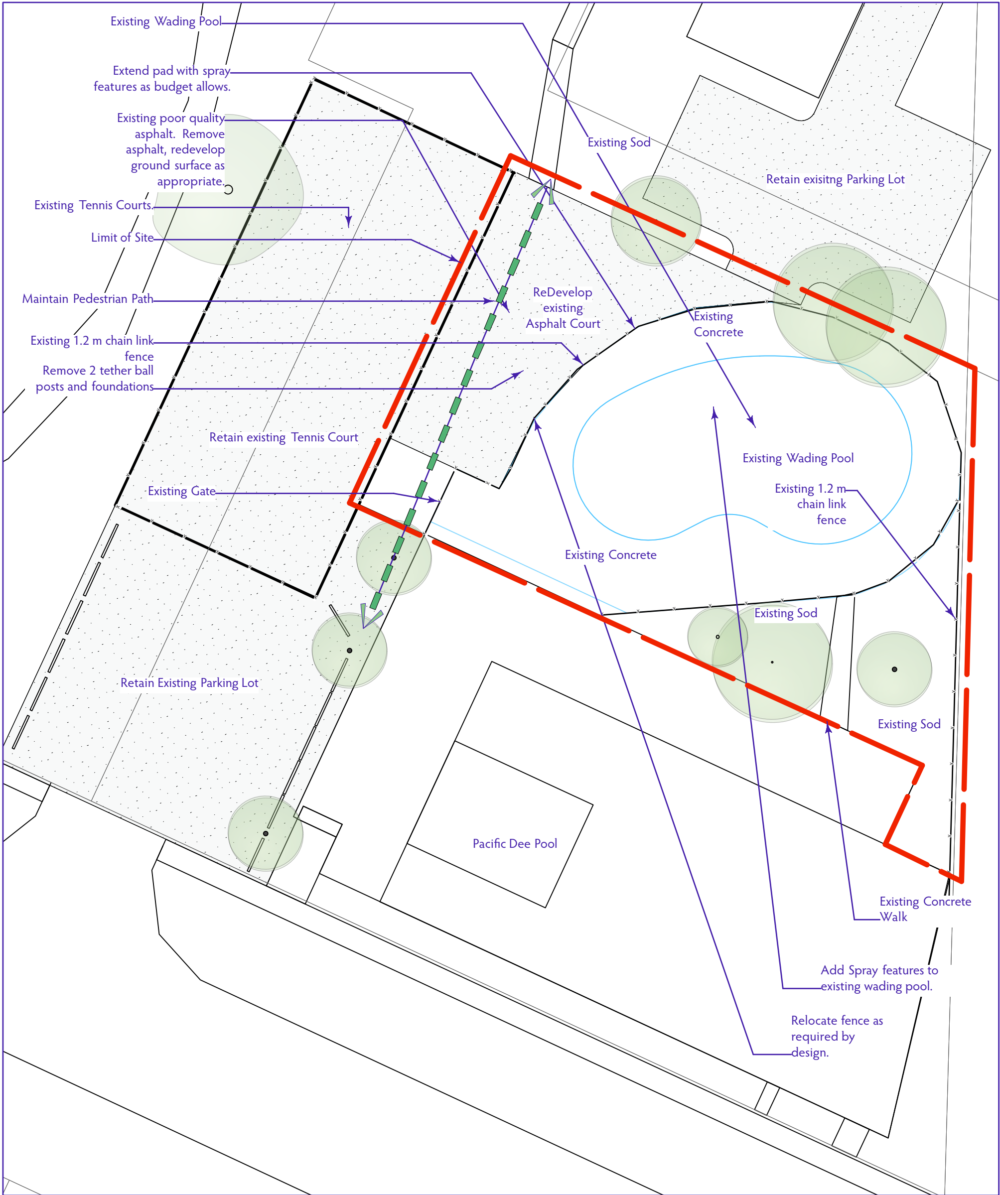
1 Site Limits Plan PD-2 Scale: 1:250
