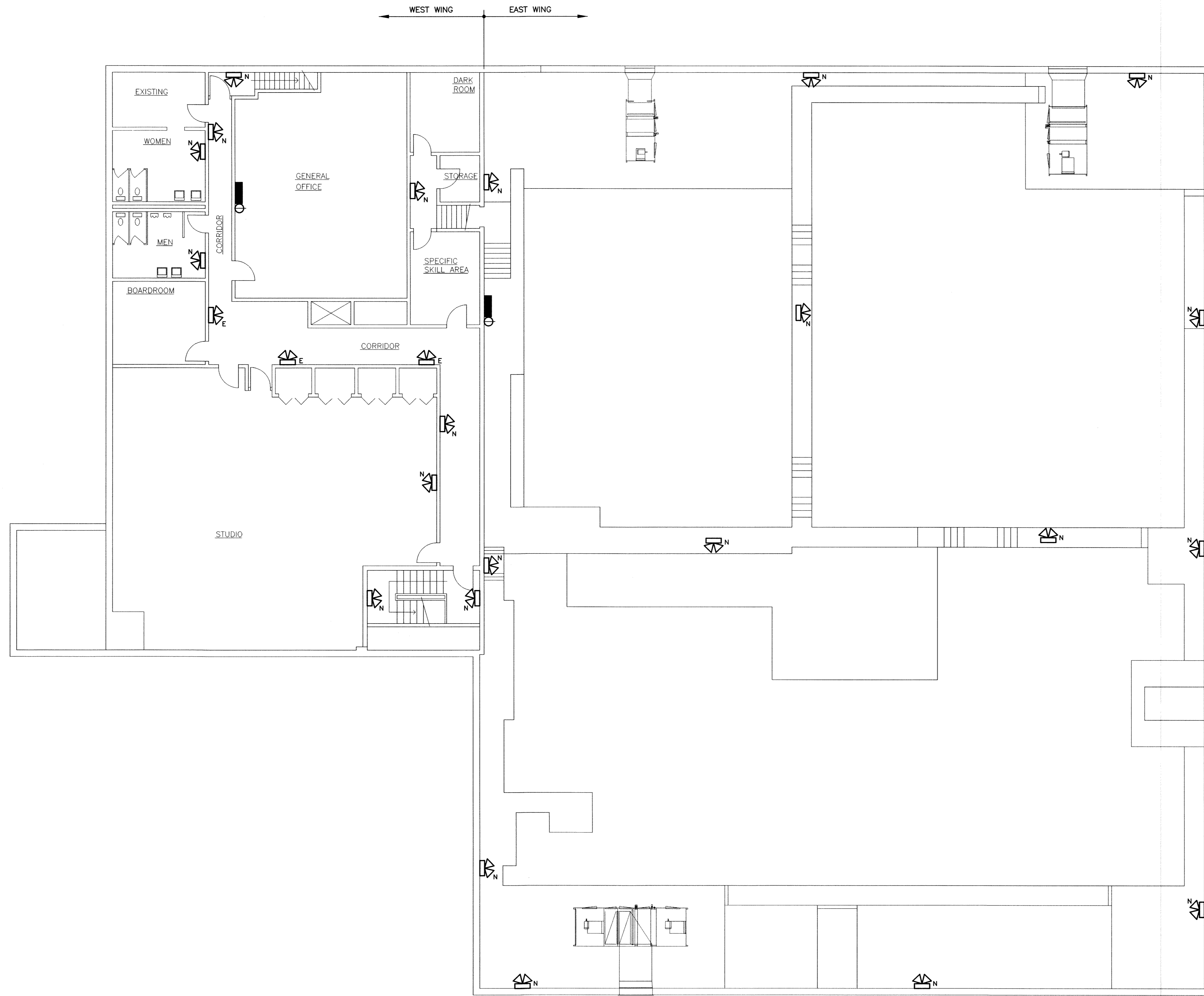
1 MEZZANINE/SECOND FLOOR PLAN 2000 0 2000 4000 6000 8000 SCALE: 1:100mm (24"x36") 1:200mm (11"x17")
