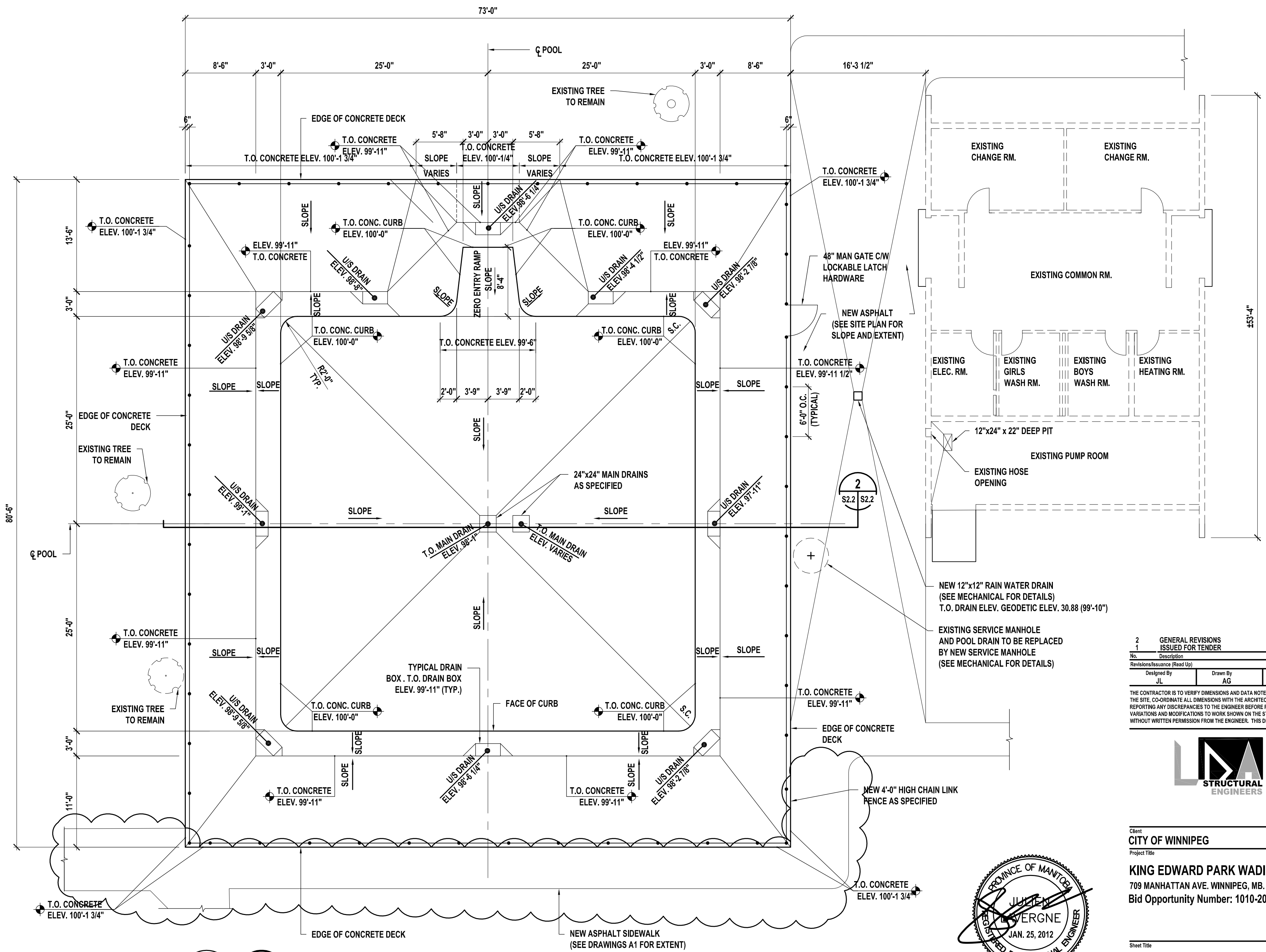
NEW POOL PLAN Scale= 1/8"=1'-0"
