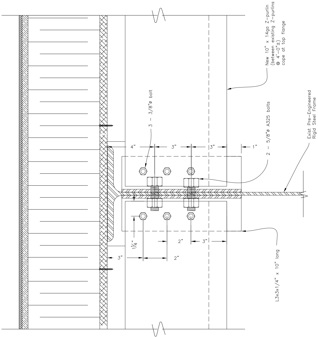
PURLIN DETAIL AT FRAME #2 SCALE: 3" = 1'-0"
