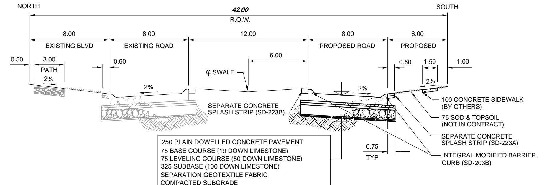
1 NTS WAVERLEY STREET CROSS SECTION (STA 10+31.3 TO STA 14+95.6)
